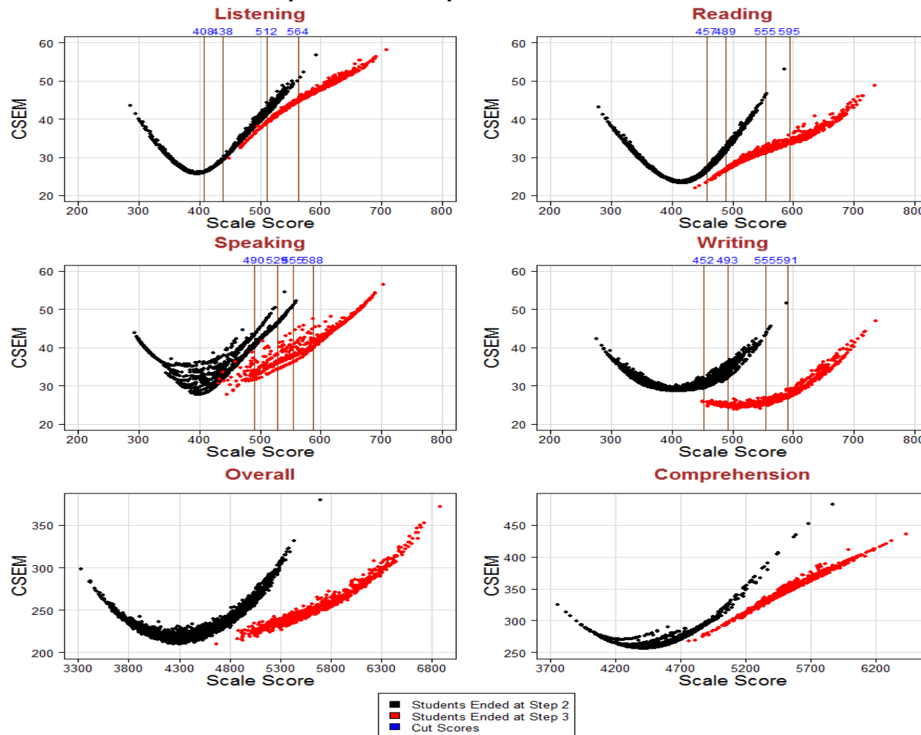
Figure S9.4: Screener Conditional Standard Error of Measurement for Grade 2
