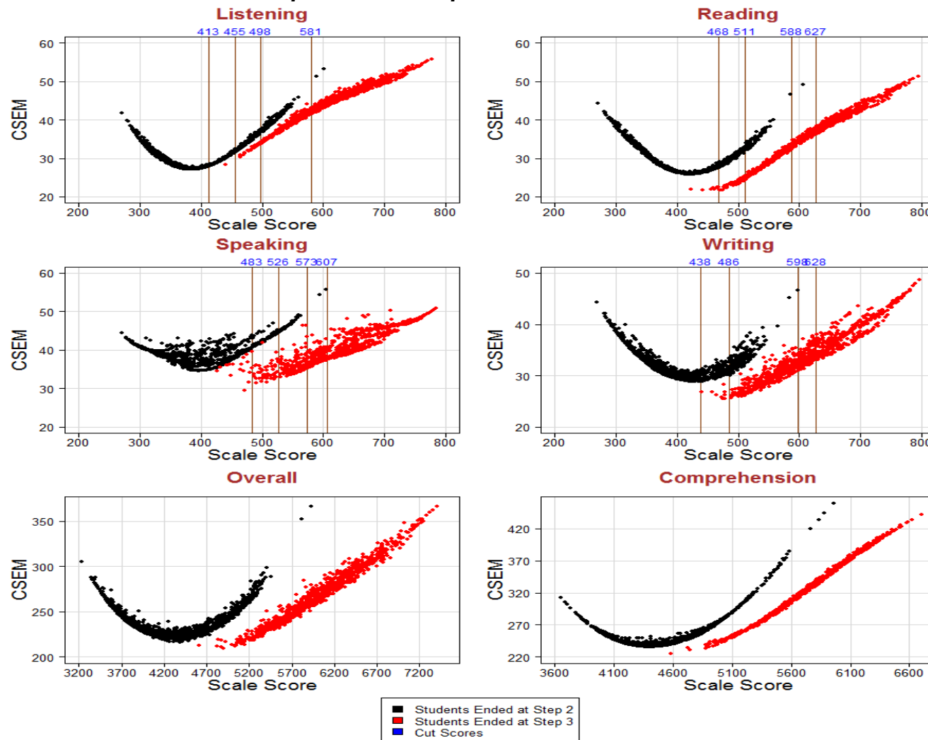
Figure S9.7: Screener Conditional Standard Error of Measurement for Grade 5
