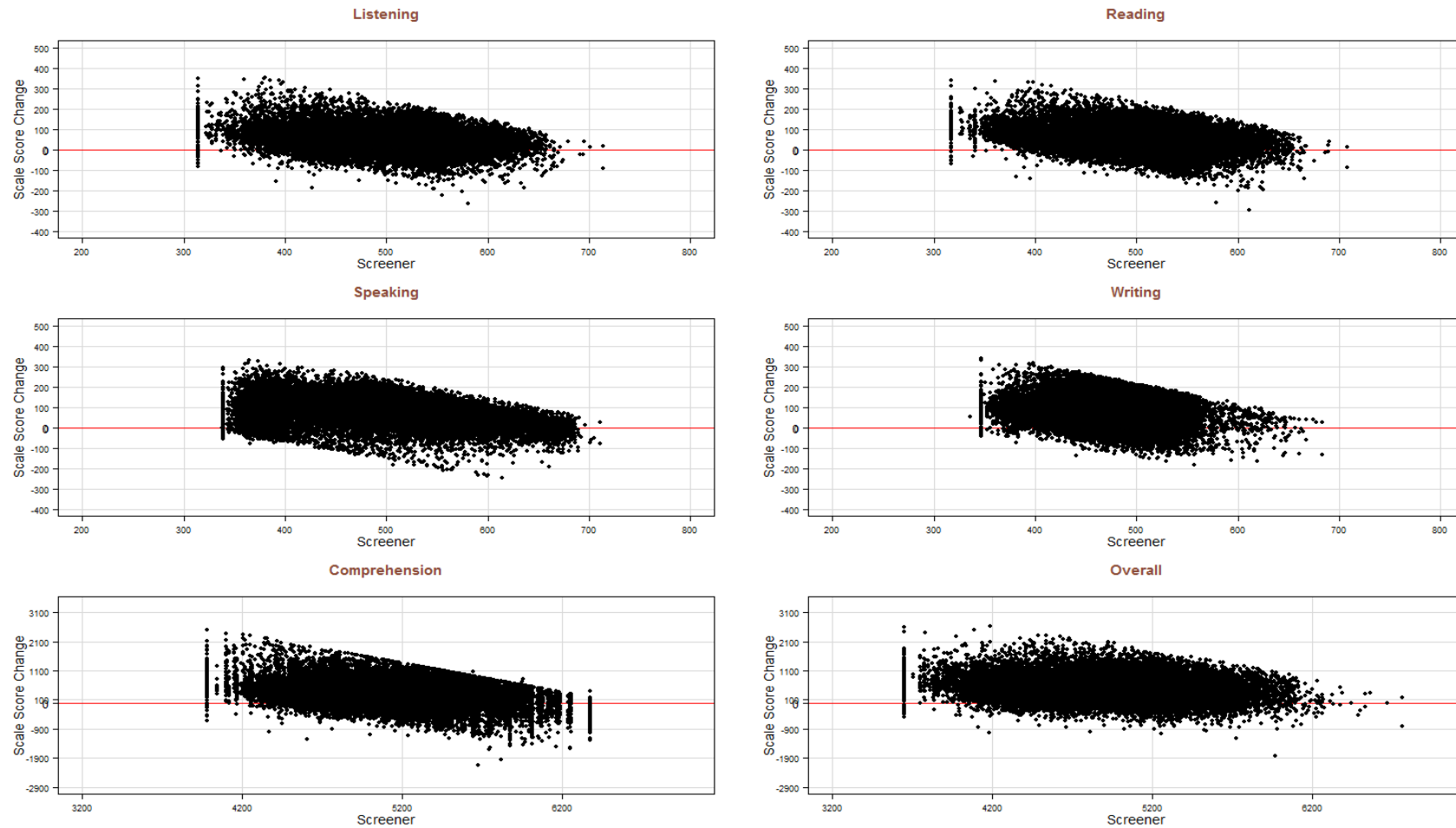
Figure S13.5: Scatter Plot of Scale Score Change from Screener to Summative for Grade K
