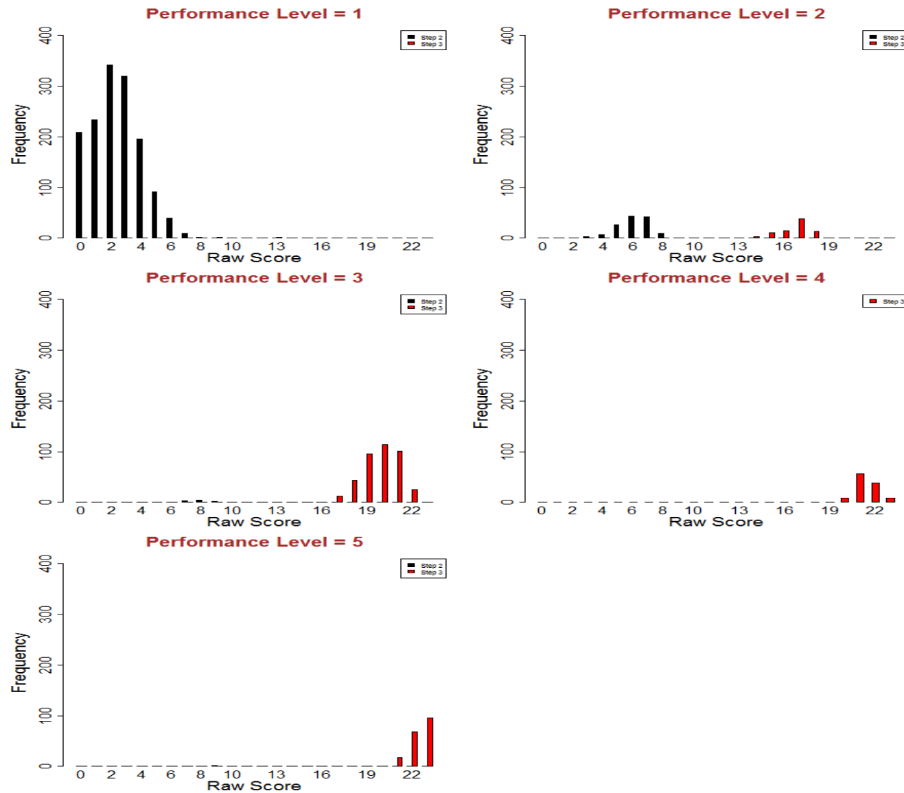
Figure S3.49: Screener Raw Score Distributions - Grade 8 Writing
