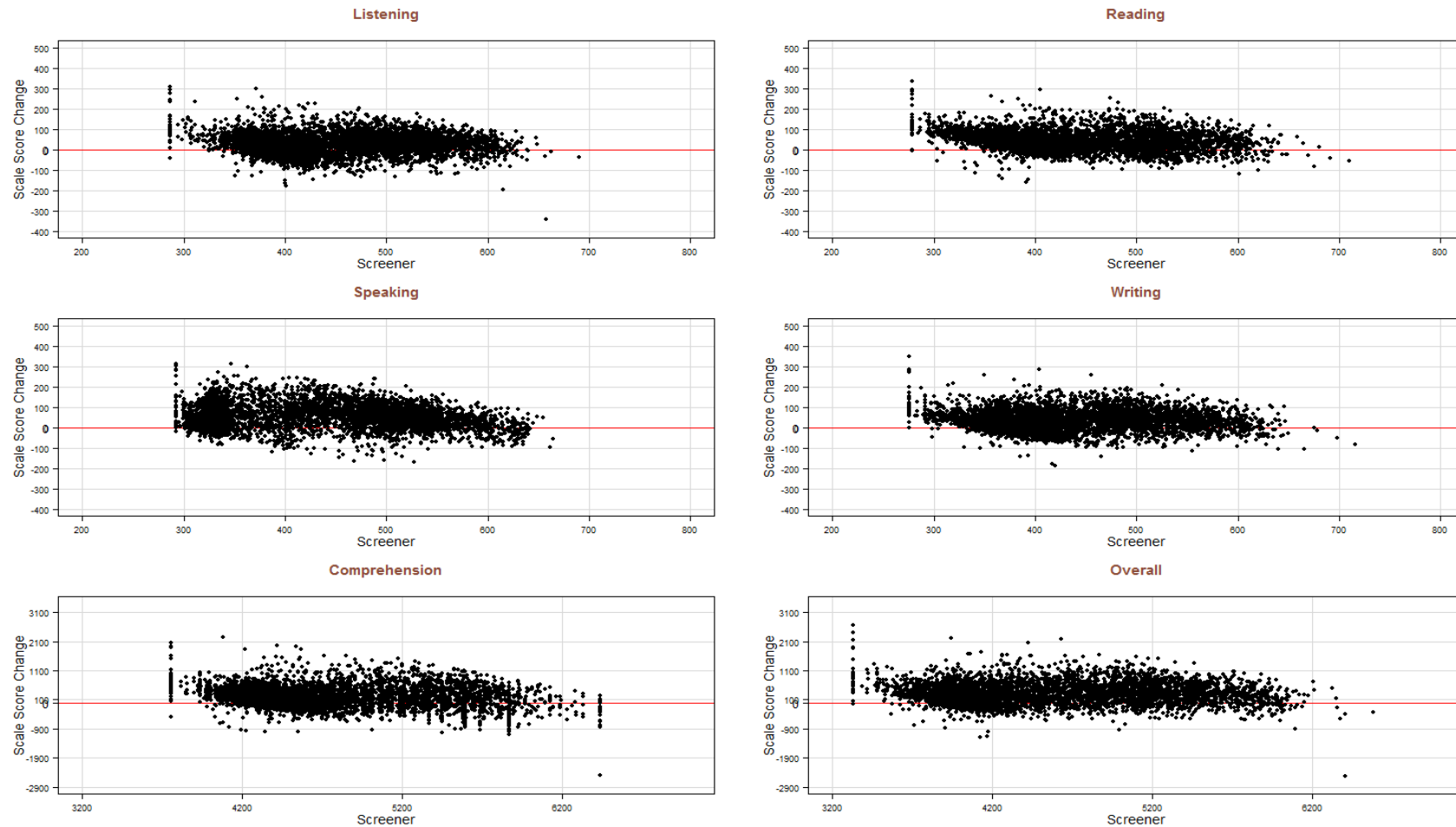
Figure S13.7: Scatter Plot of Scale Score Change from Screener to Summative for Grade Band 2-3
