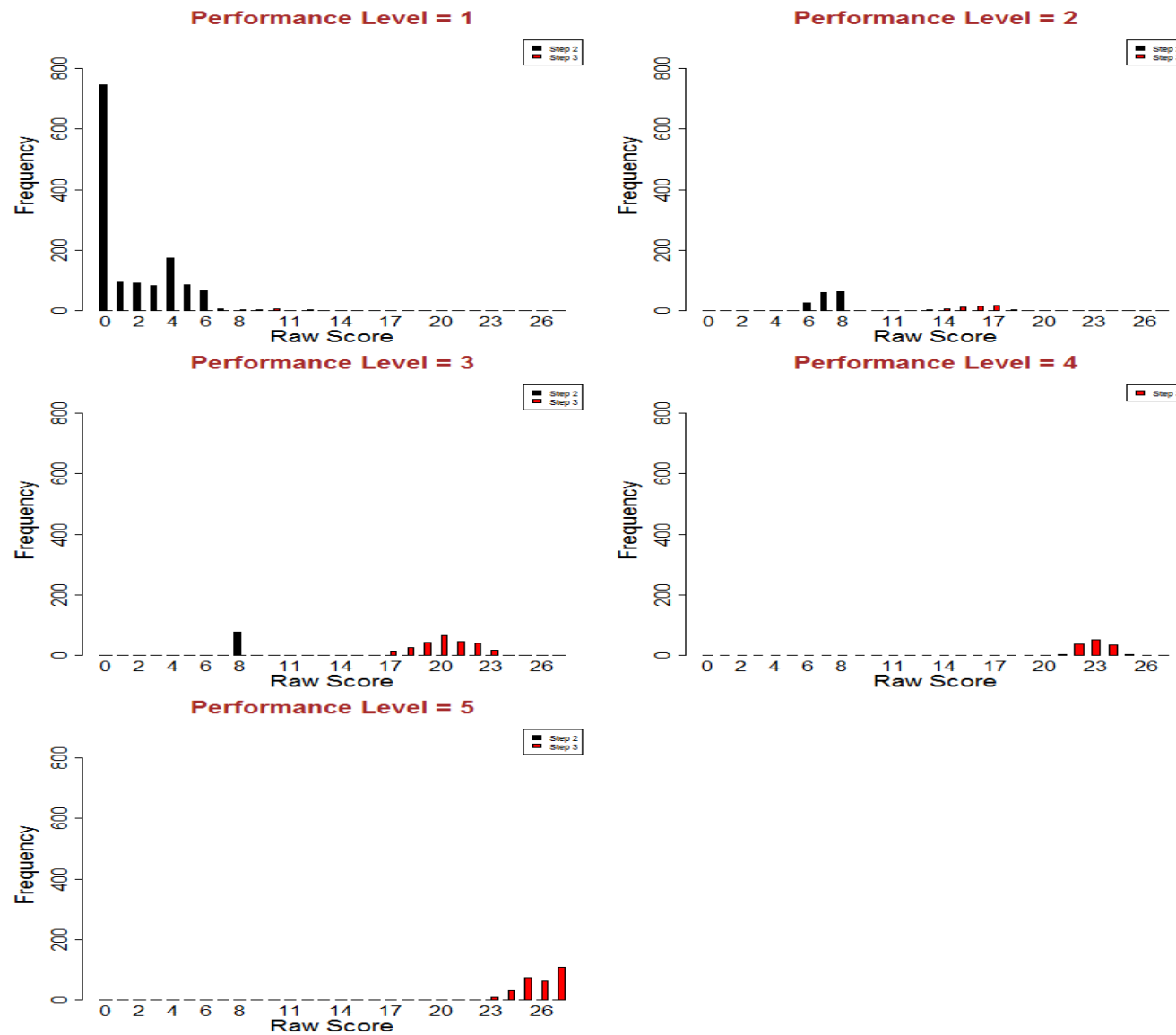
Figure S3.48: Screener Raw Score Distributions - Grade 8 Speaking
