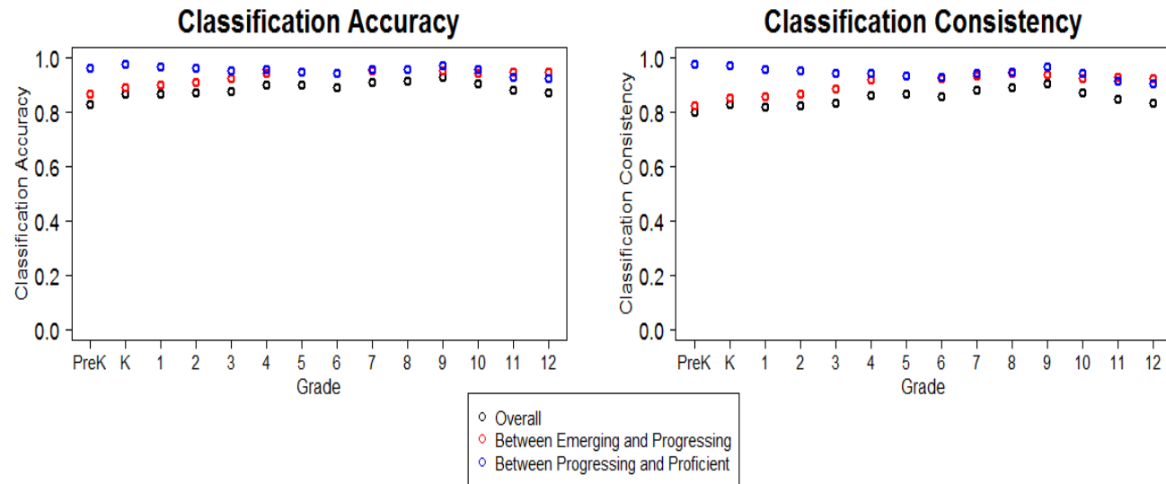
Figure S10.3: Screener Overall Proficiency Classification
