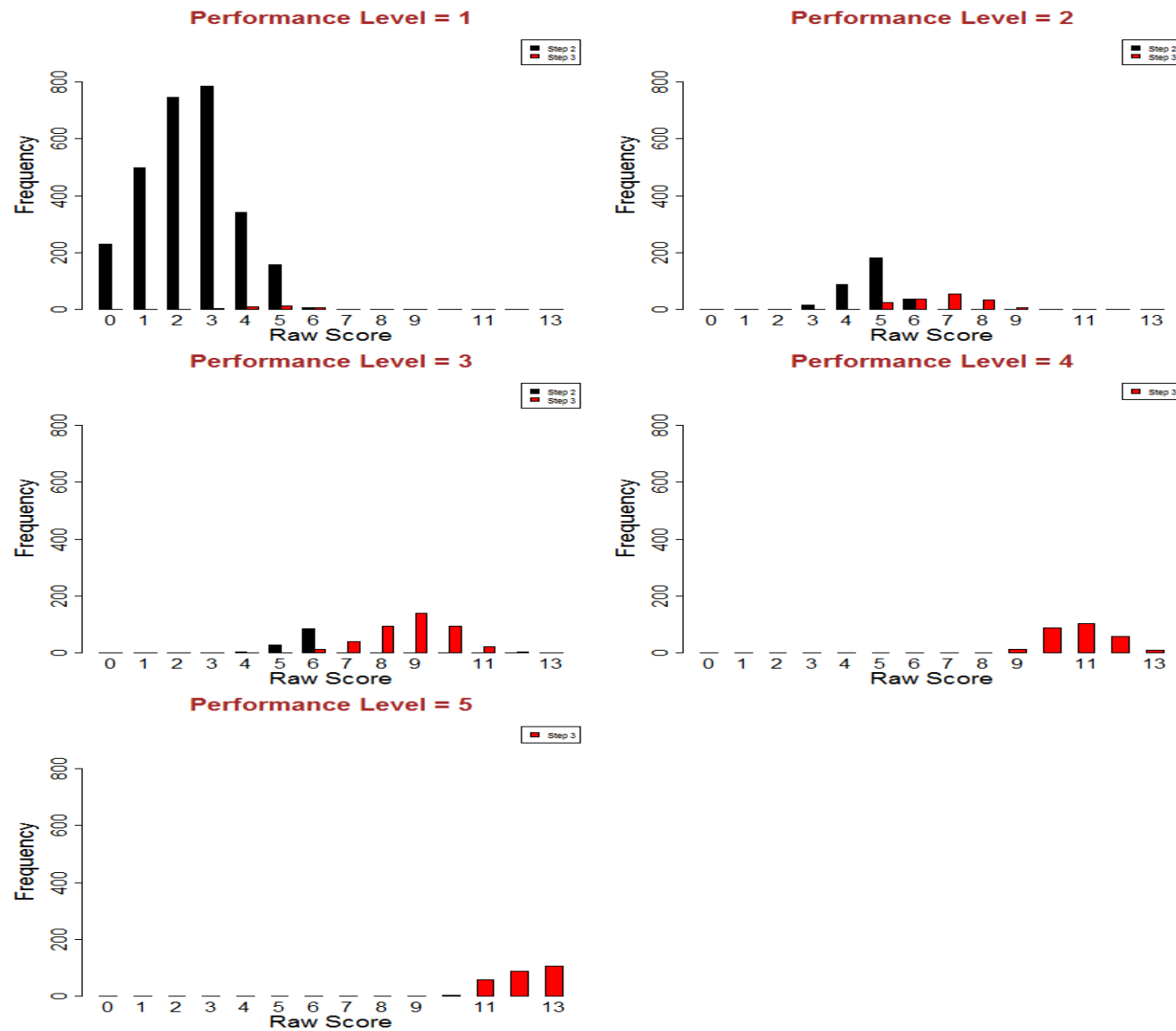
Figure S3.12: Screener Raw Score Distributions - Grade 1 Reading
