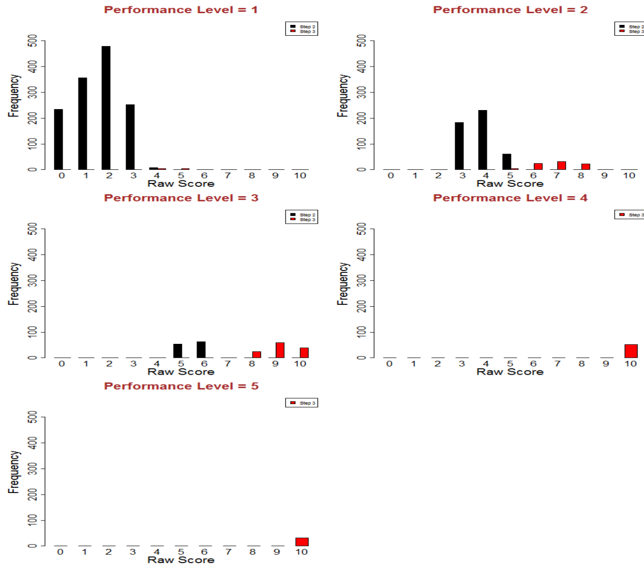
Figure S3.9: Screener Raw Score Distributions - Kindergarten Writing
