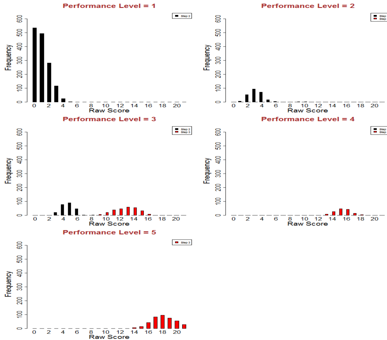
Figure S3.29: Screener Raw Score Distributions - Grade 4 Writing
