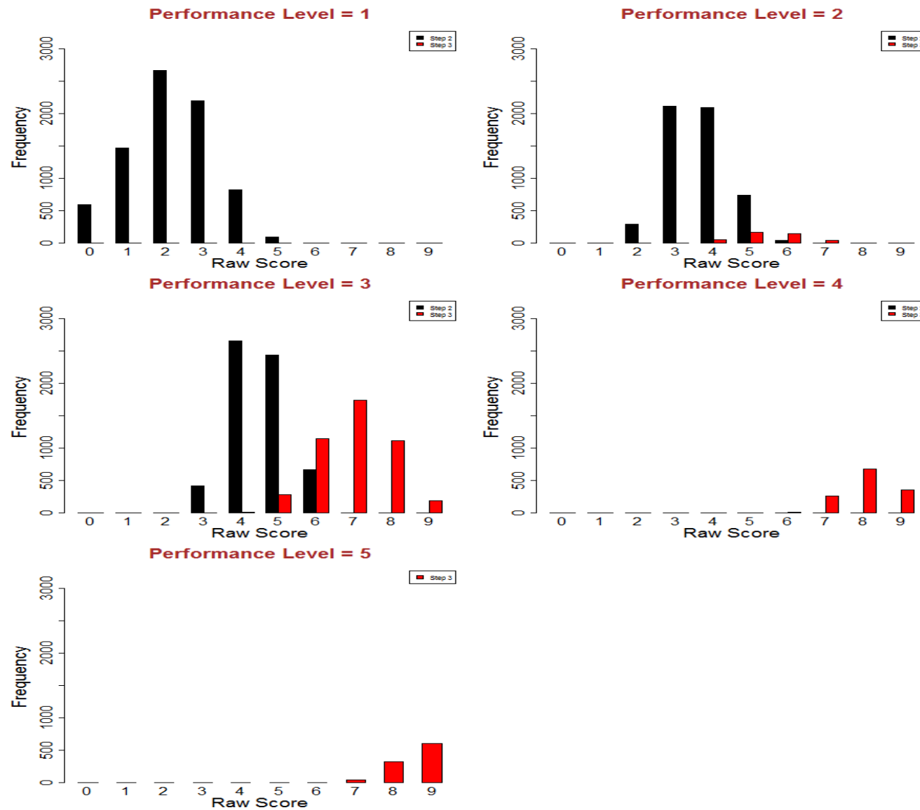
Figure S3.2: Screener Raw Score Distributions - Pre-Kindergarten Reading
