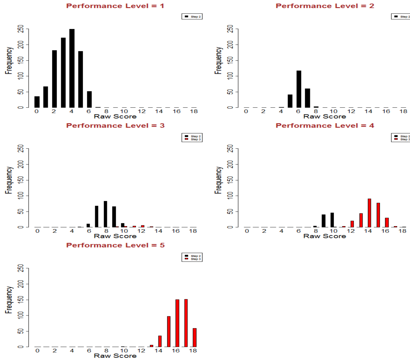
Figure S3.36: Screener Raw Score Distributions - Grade 6 Listening
