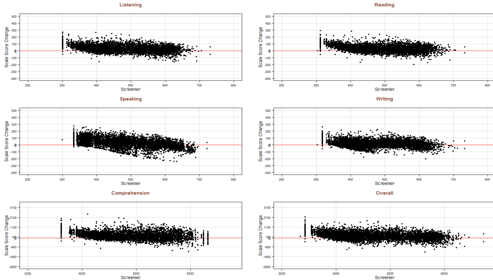
Figure S13.10: Scatter Plot of Scale Score Change from Screener to Summative for Grade Band 9-12
