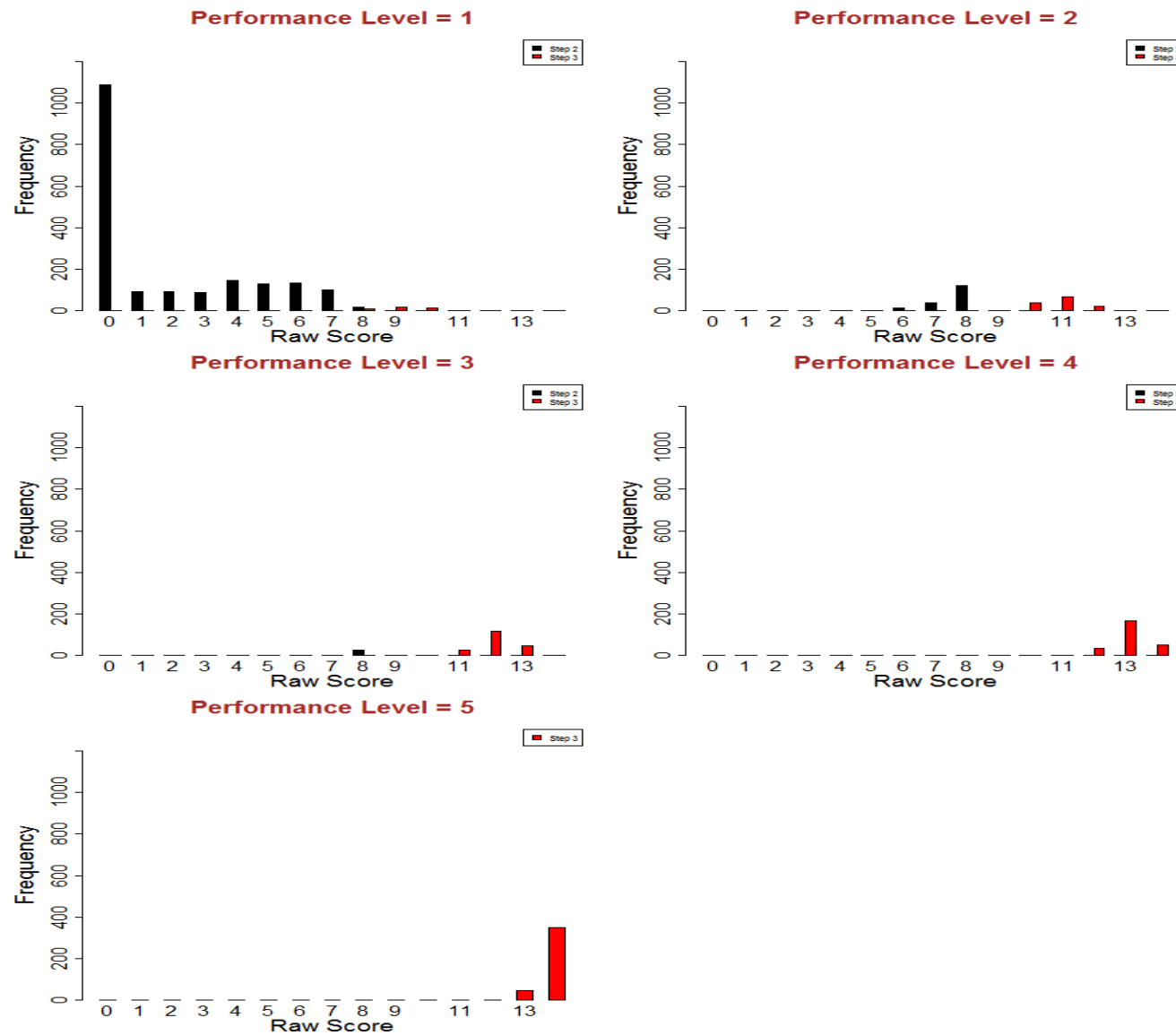
Figure S3.23: Screener Raw Score Distributions - Grade 3 Speaking
