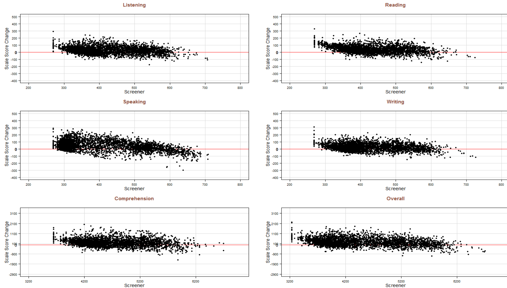
Figure S13.8: Scatter Plot of Scale Score Change from Screener to Summative for Grade Band 4-5
