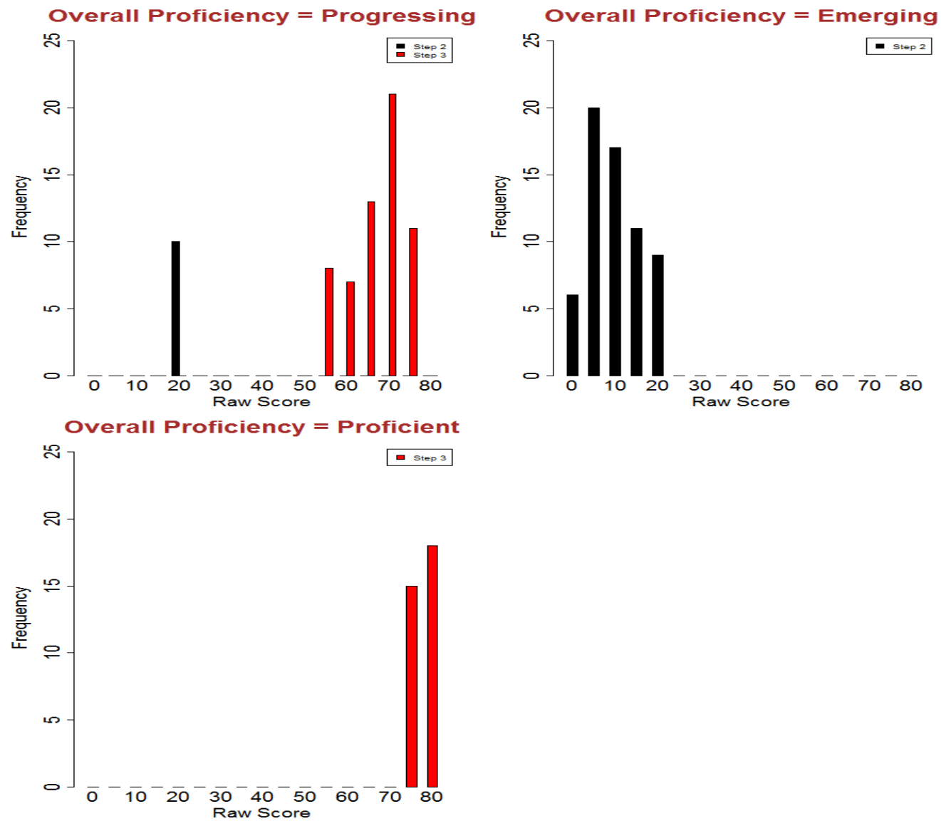
Figure S3.70: Screener Raw Score Distributions - Grade 12 Overall
