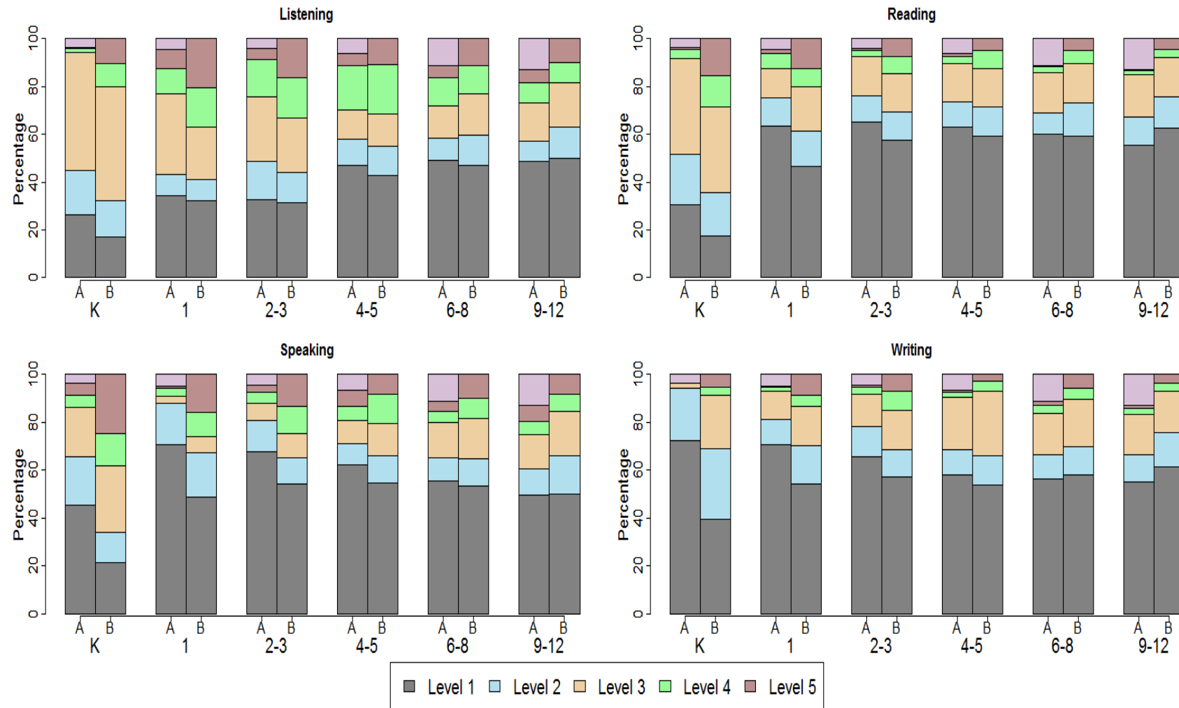
Figure S13.3: Percentages of Domain Performance Level Progress
