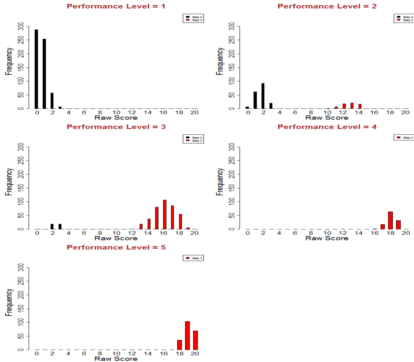
Figure S3.64: Screener Raw Score Distributions - Grade 11 Writing
