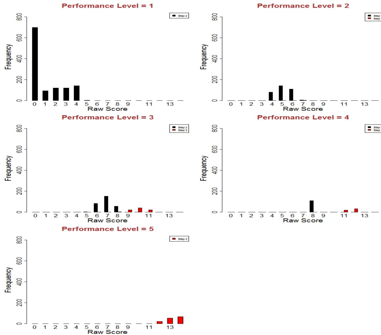
Figure S3.8: Screener Raw Score Distributions - Kindergarten Speaking
