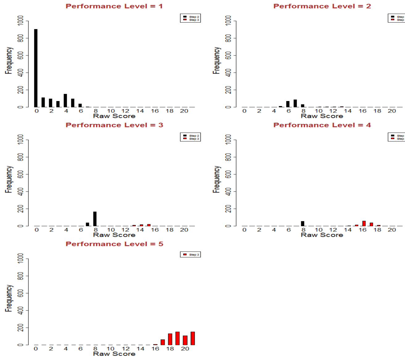
Figure S3.28: Screener Raw Score Distributions - Grade 4 Speaking
