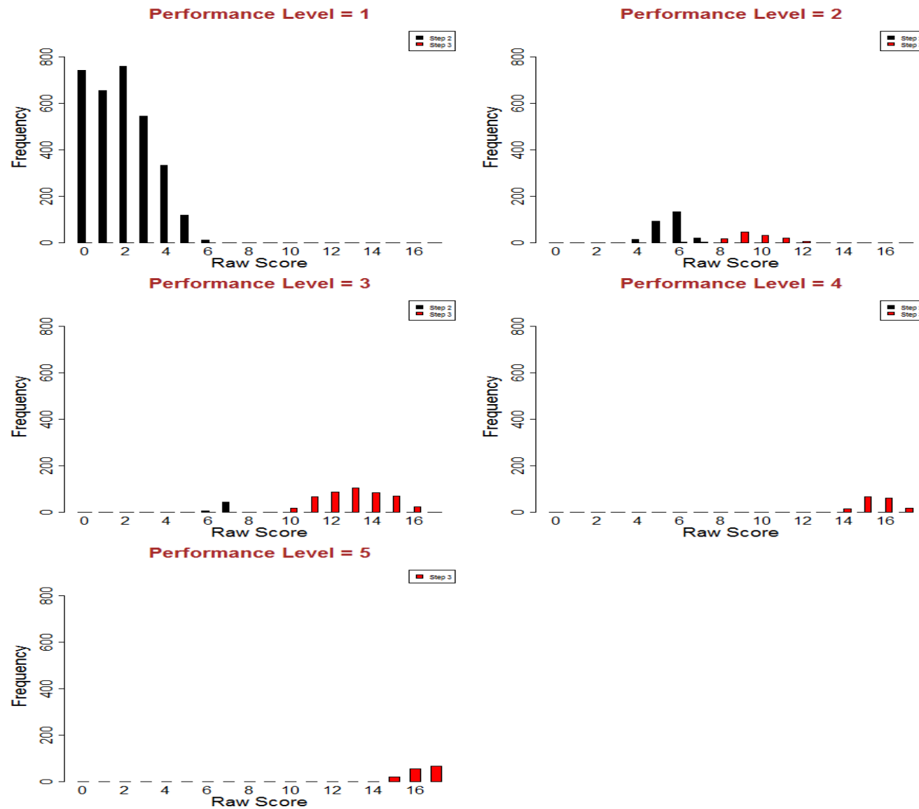
Figure S3.52: Screener Raw Score Distributions - Grade 9 Reading
