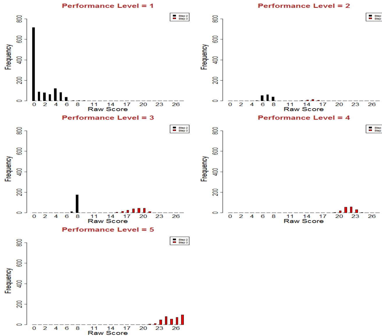
Figure S3.38: Screener Raw Score Distributions - Grade 6 Speaking
