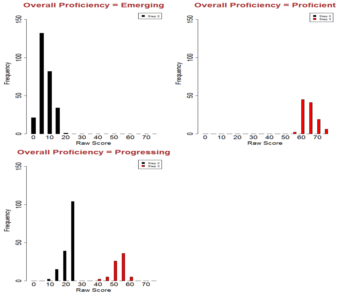
Figure S3.30: Screener Raw Score Distributions - Grade 4 Overall
