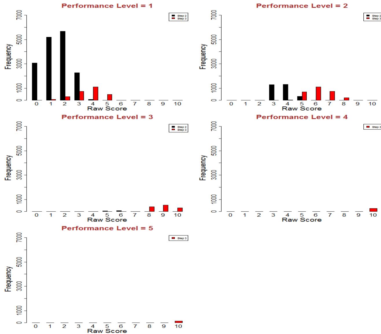
Figure S3.4: Screener Raw Score Distributions - Pre-Kindergarten Writing
