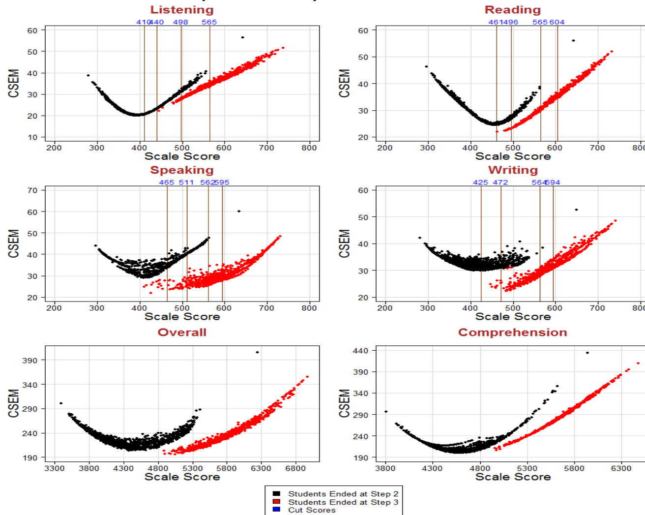
Figure S9.8: Screener Conditional Standard Error of Measurement for Grade 6
