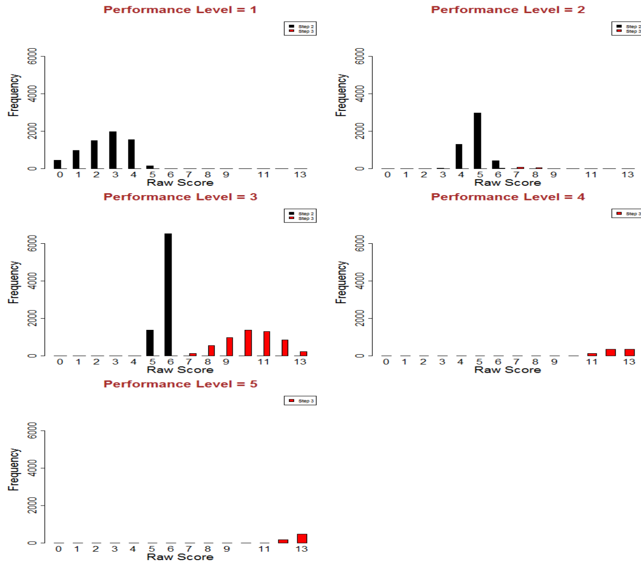
Figure S3.1: Screener Raw Score Distributions- Pre-Kindergarten Listening
