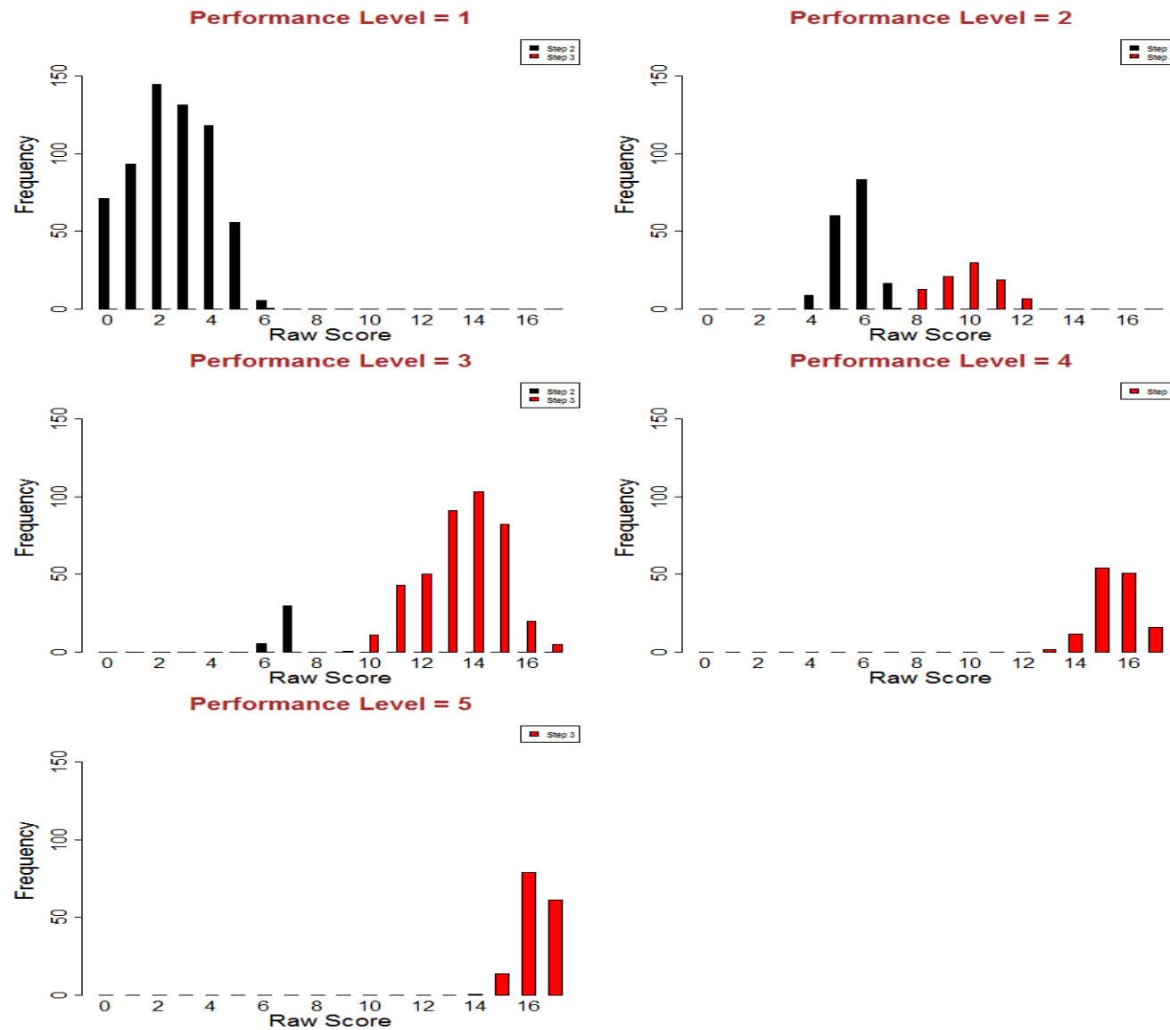
Figure S3.62: Screener Raw Score Distributions - Grade 11 Reading
