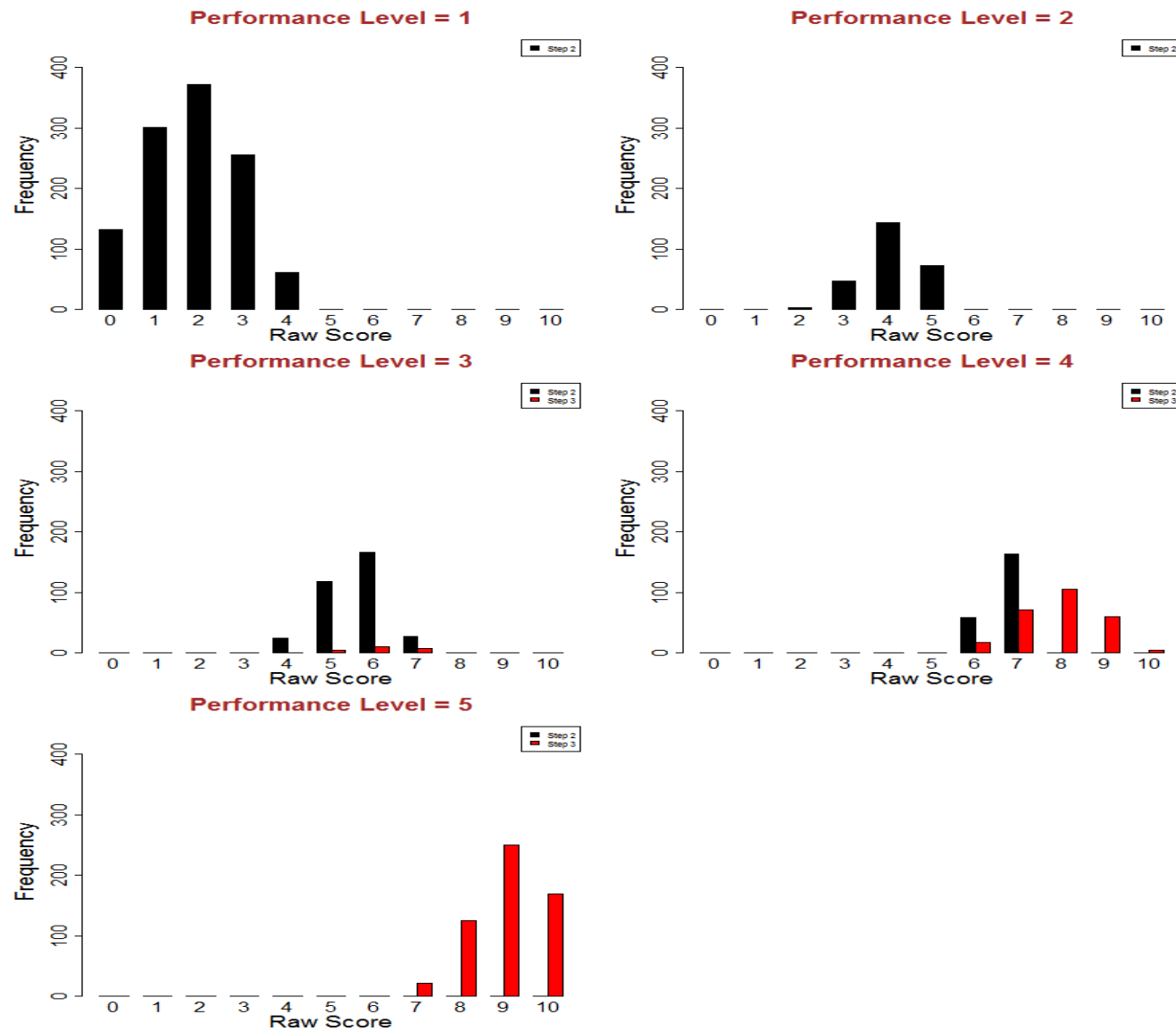
Figure S3.26: Screener Raw Score Distributions - Grade 4 Listening
