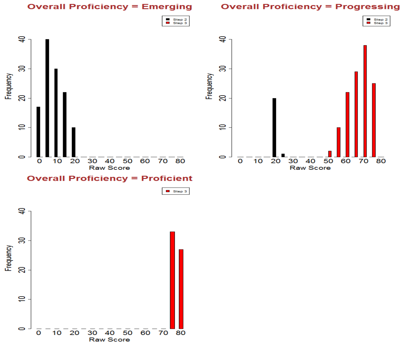
Figure S3.65: Screener Raw Score Distributions - Grade 11 Overall
