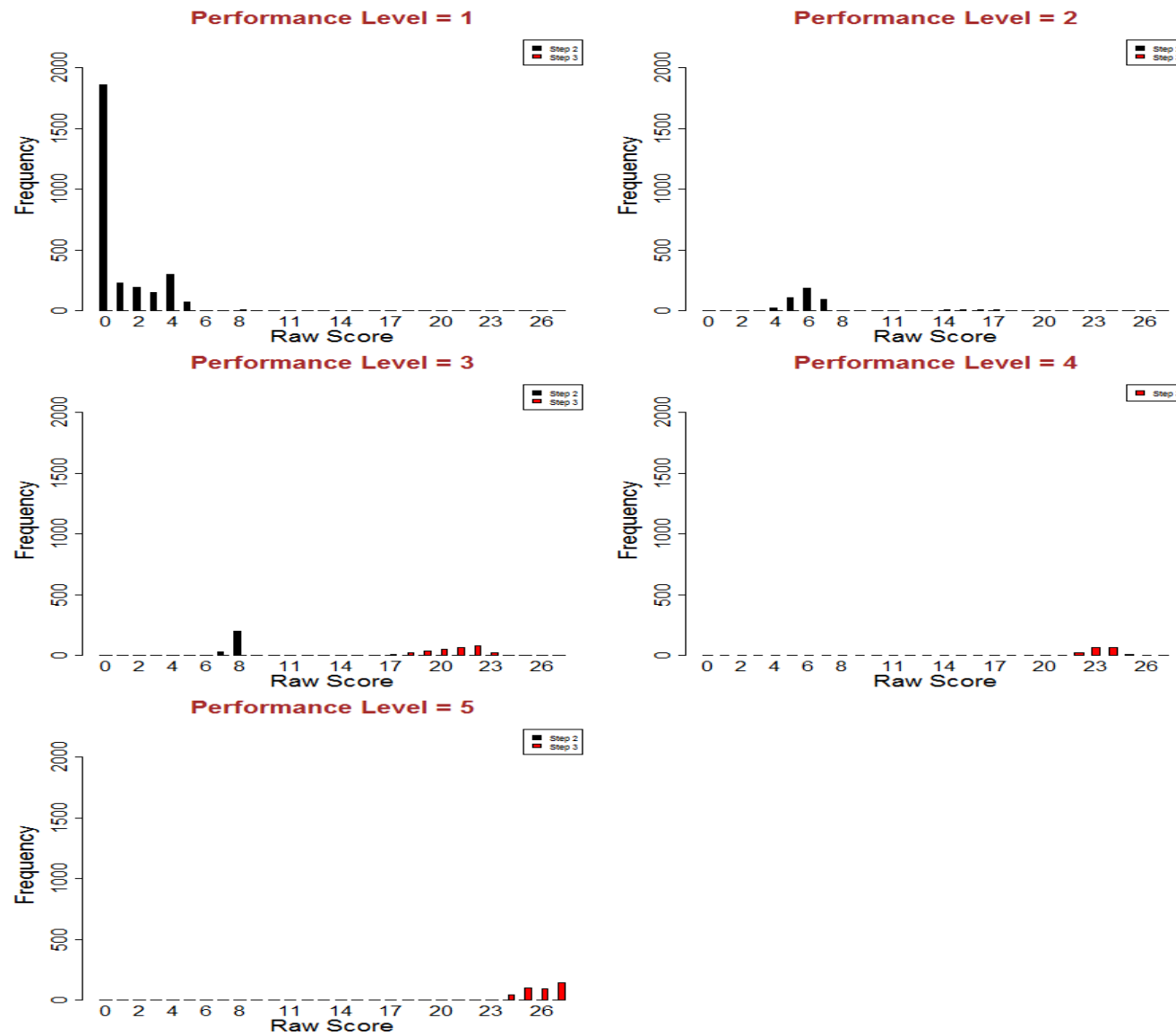
Figure S3.53: Screener Raw Score Distributions - Grade 9 Speaking
