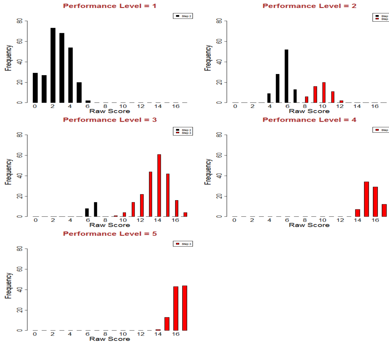
Figure S3.67: Screener Raw Score Distributions - Grade 12 Reading
