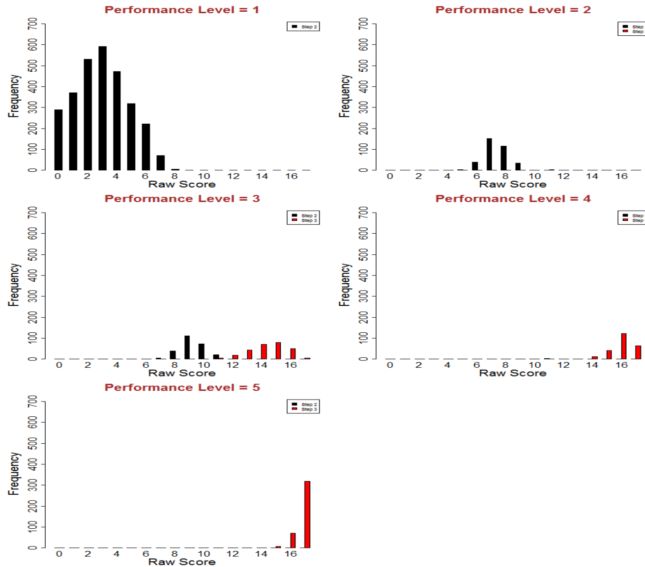
Figure S3.51: Screener Raw Score Distributions - Grade 9 Listening
