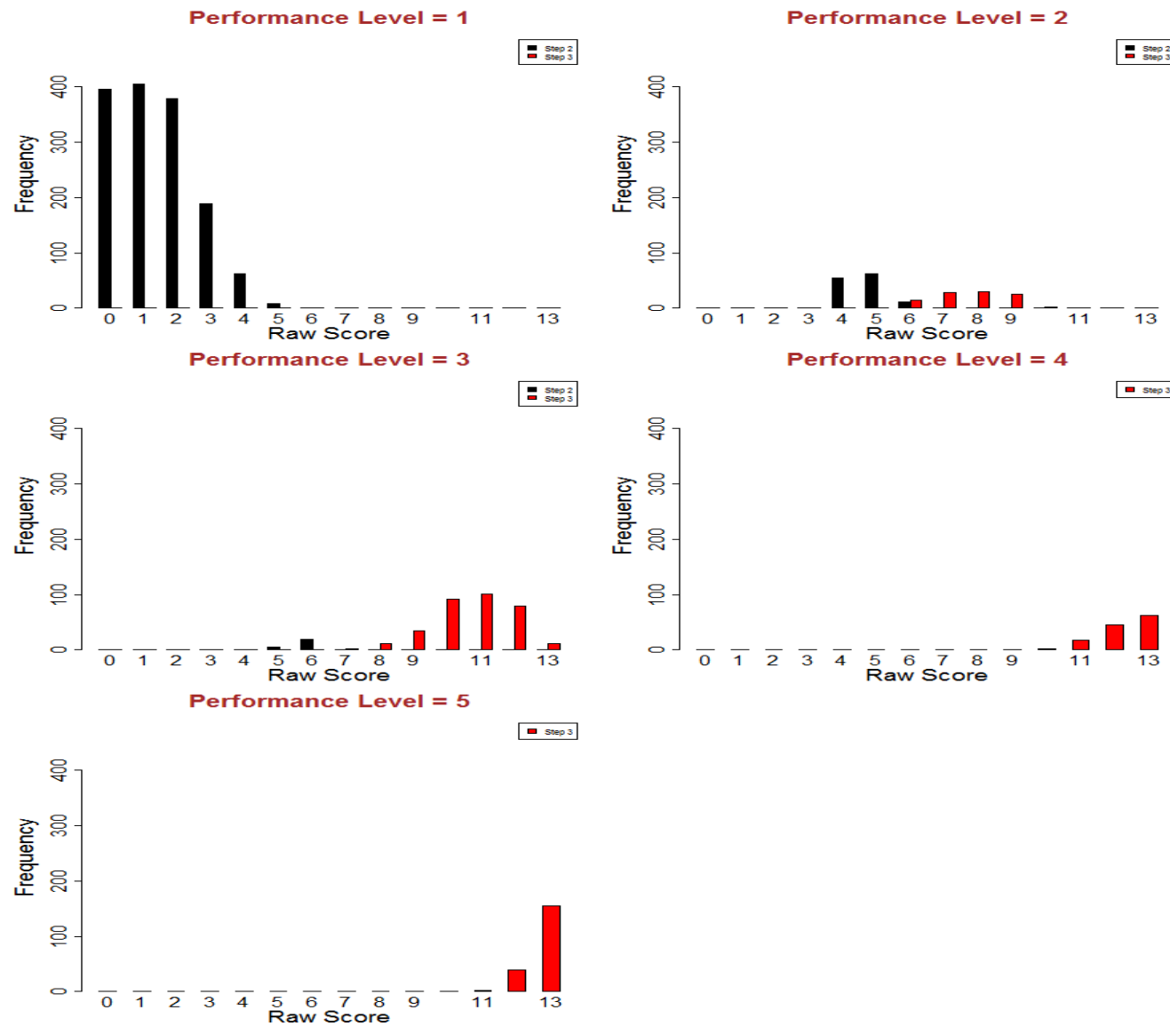
Figure S3.42: Screener Raw Score Distributions - Grade 7 Reading
