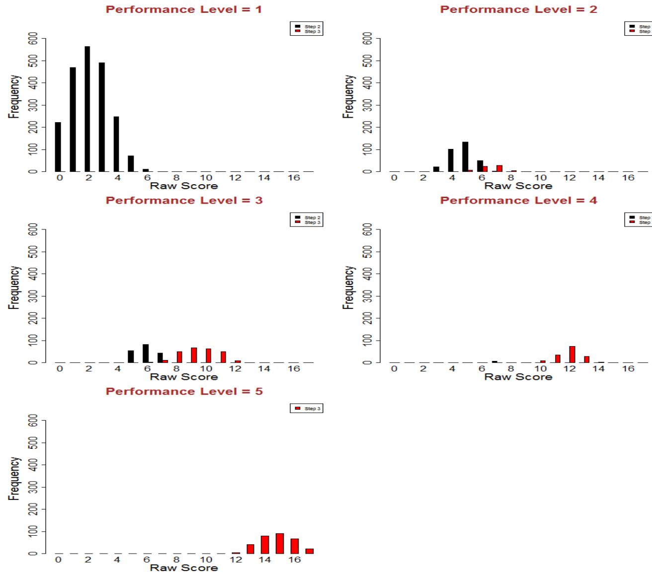
Figure S3.19: Screener Raw Score Distributions - Grade 2 Writing
