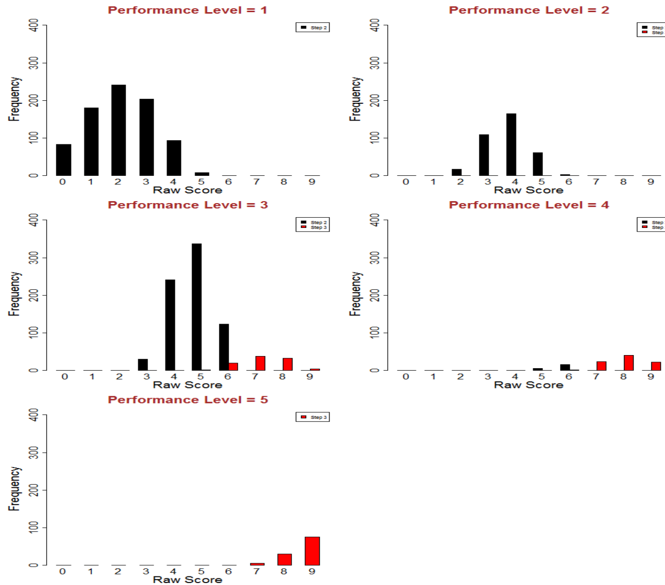
Figure S3.7: Screener Raw Score Distributions - Kindergarten Reading
