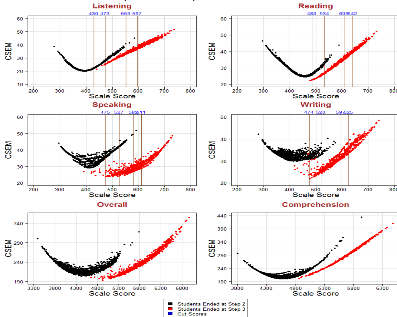
Figure S9.9: Screener Conditional Standard Error of Measurement for Grade 7
