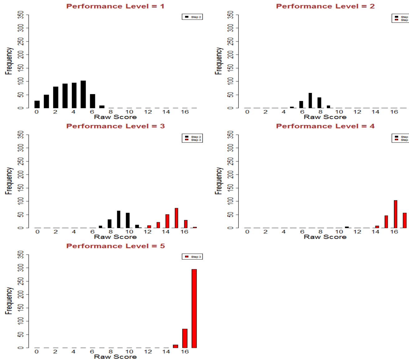
Figure S3.61: Screener Raw Score Distributions - Grade 11 Listening
