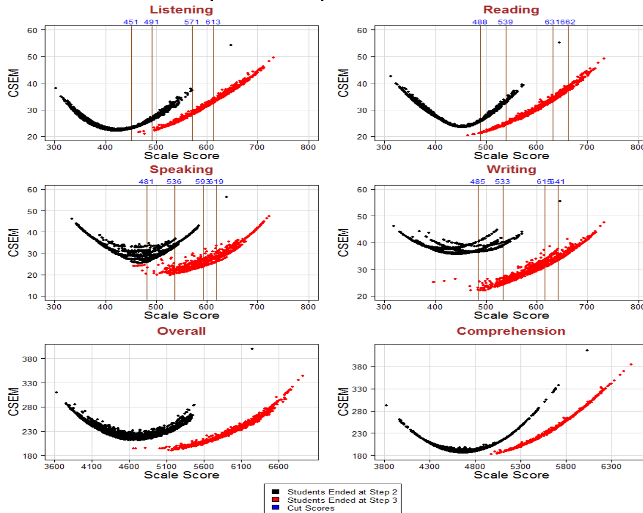
Figure S9.11: Screener Conditional Standard Error of Measurement for Grade 9
