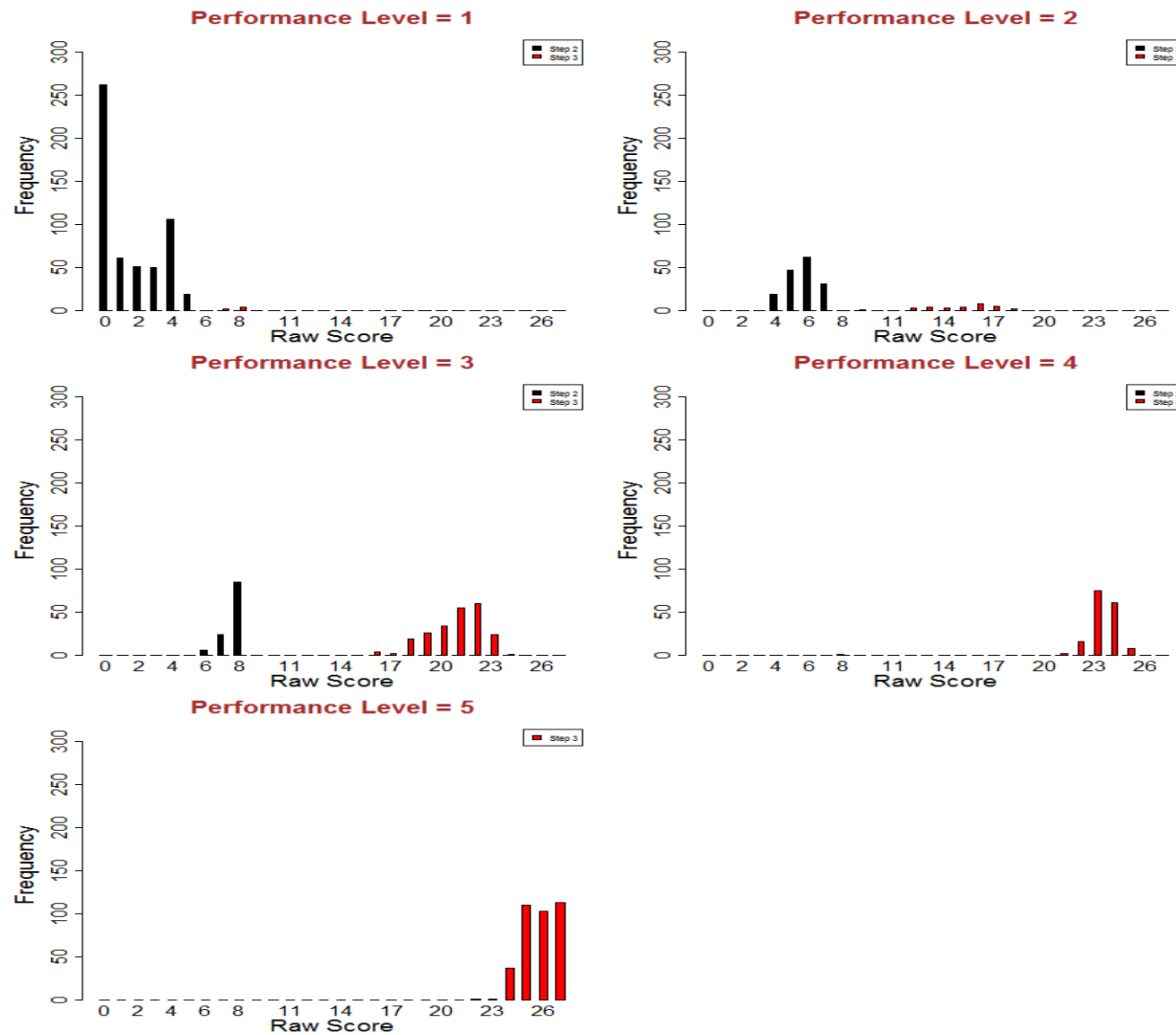
Figure S3.63: Screener Raw Score Distributions - Grade 11 Speaking
