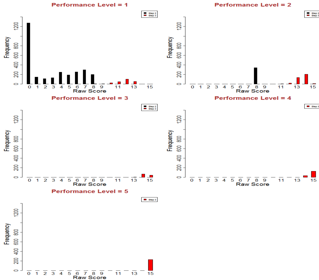
Figure S3.13: Screener Raw Score Distributions - Grade 1 Speaking
