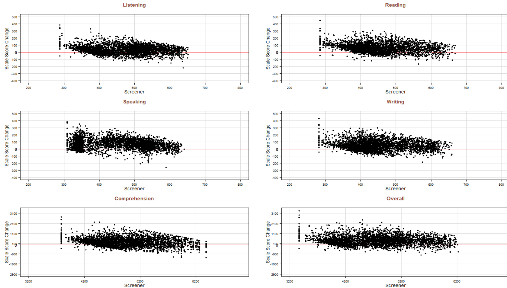
Figure S13.6: Scatter Plot of Scale Score Change from Screener to Summative for Grade 1
