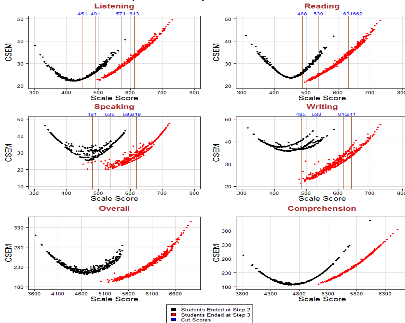
Figure S9.14: Screener Conditional Standard Error of Measurement for Grade 12
