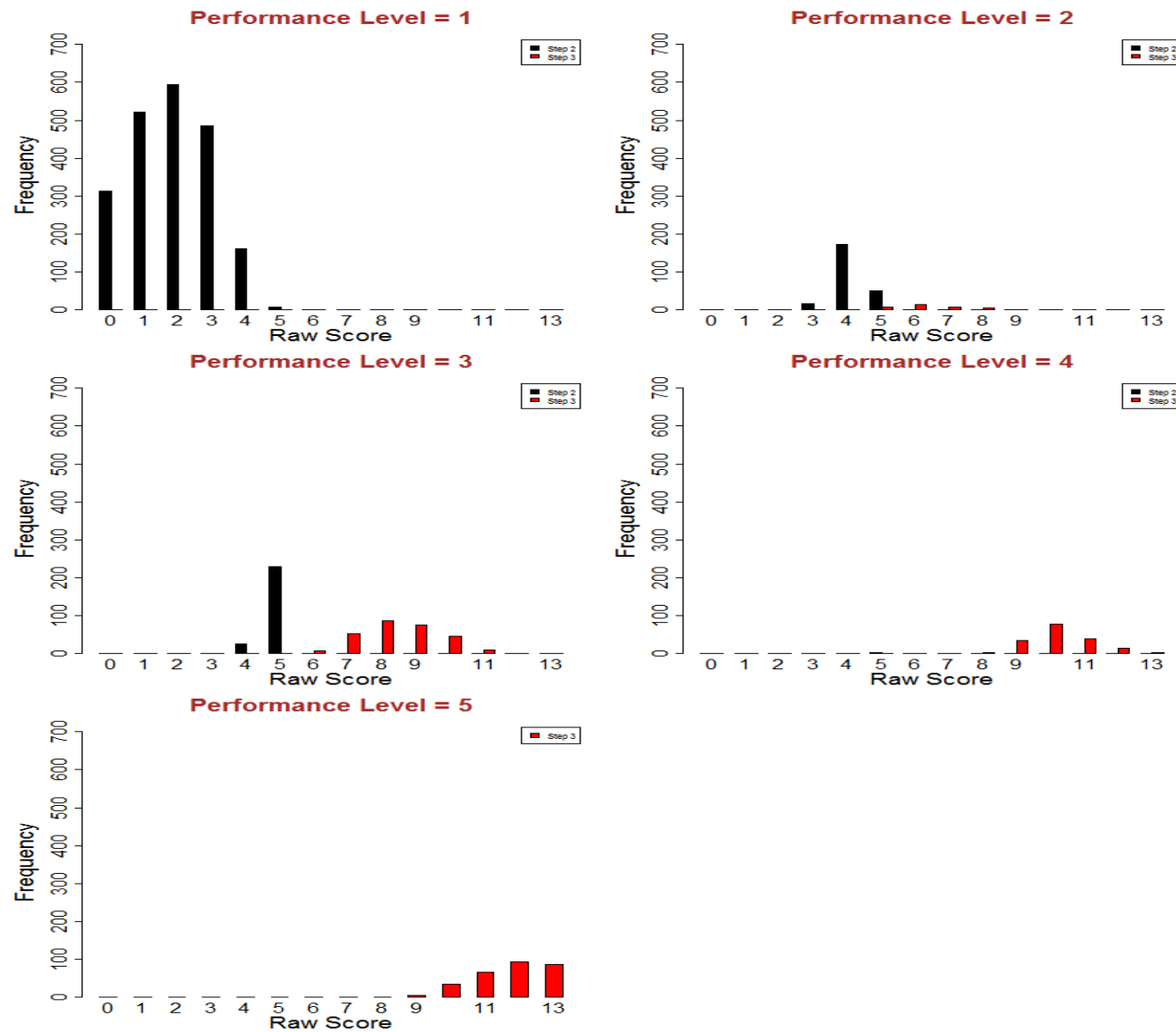
Figure S3.17: Screener Raw Score Distributions - Grade 2 Reading
