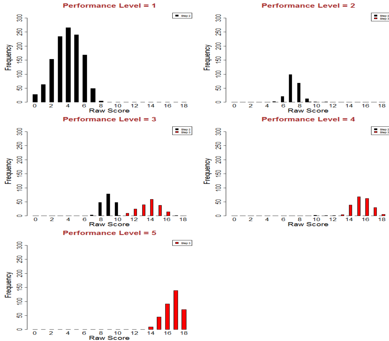
Figure S3.41: Screener Raw Score Distributions - Grade 7 Listening
