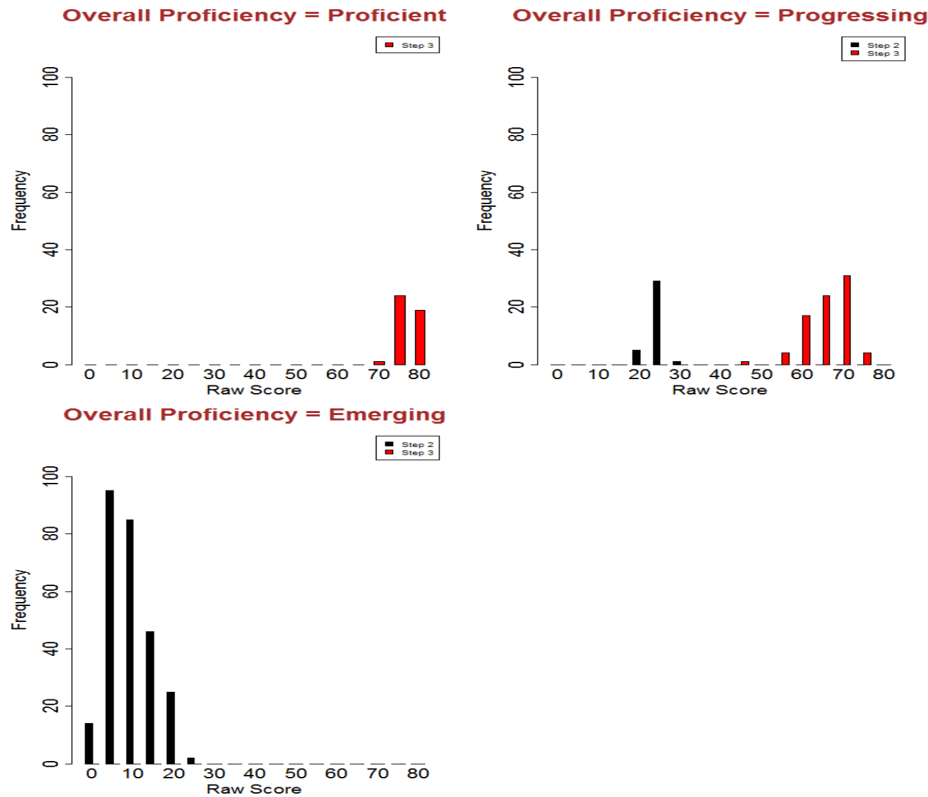
Figure S3.45: Screener Raw Score Distributions - Grade 7 Overall
