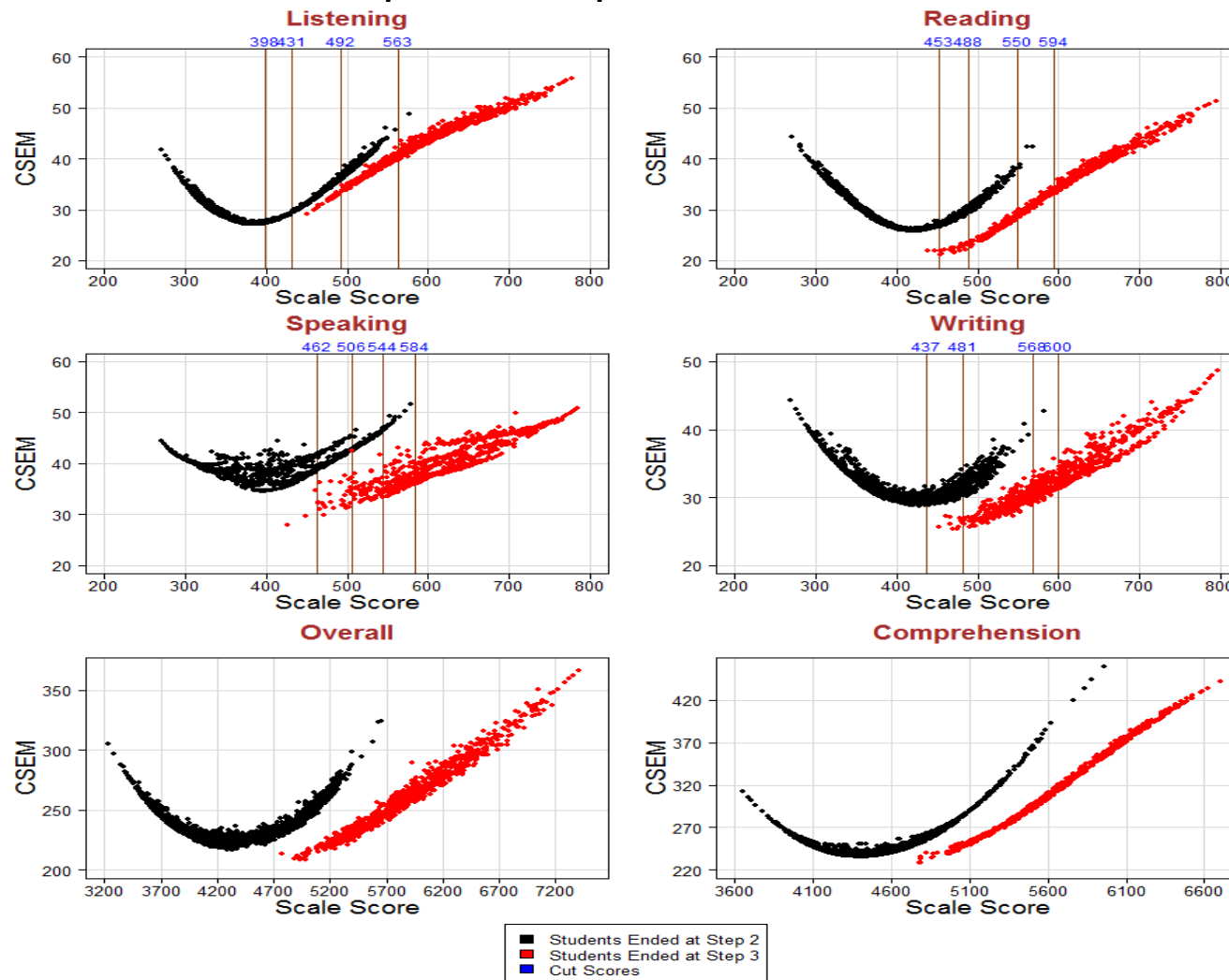
Figure S9.6: Screener Conditional Standard Error of Measurement for Grade 4
