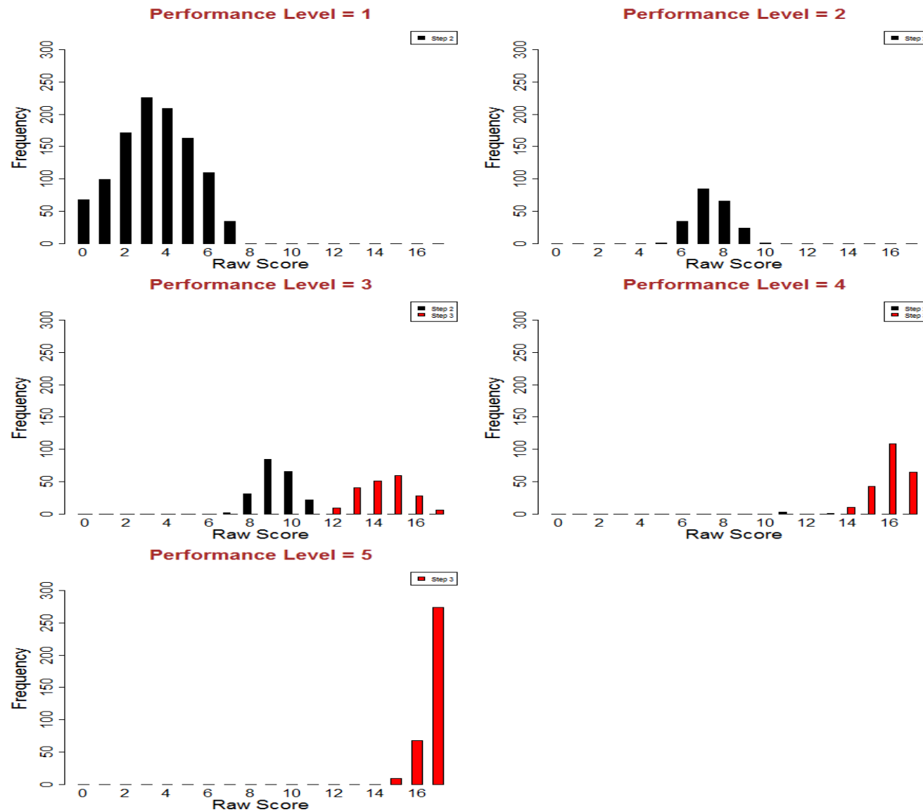
Figure S3.56: Screener Raw Score Distributions - Grade 10 Listening
