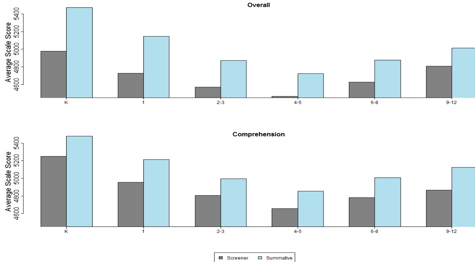
Figure S13.2: Average Overall and Comprehension Scale Score Progress
