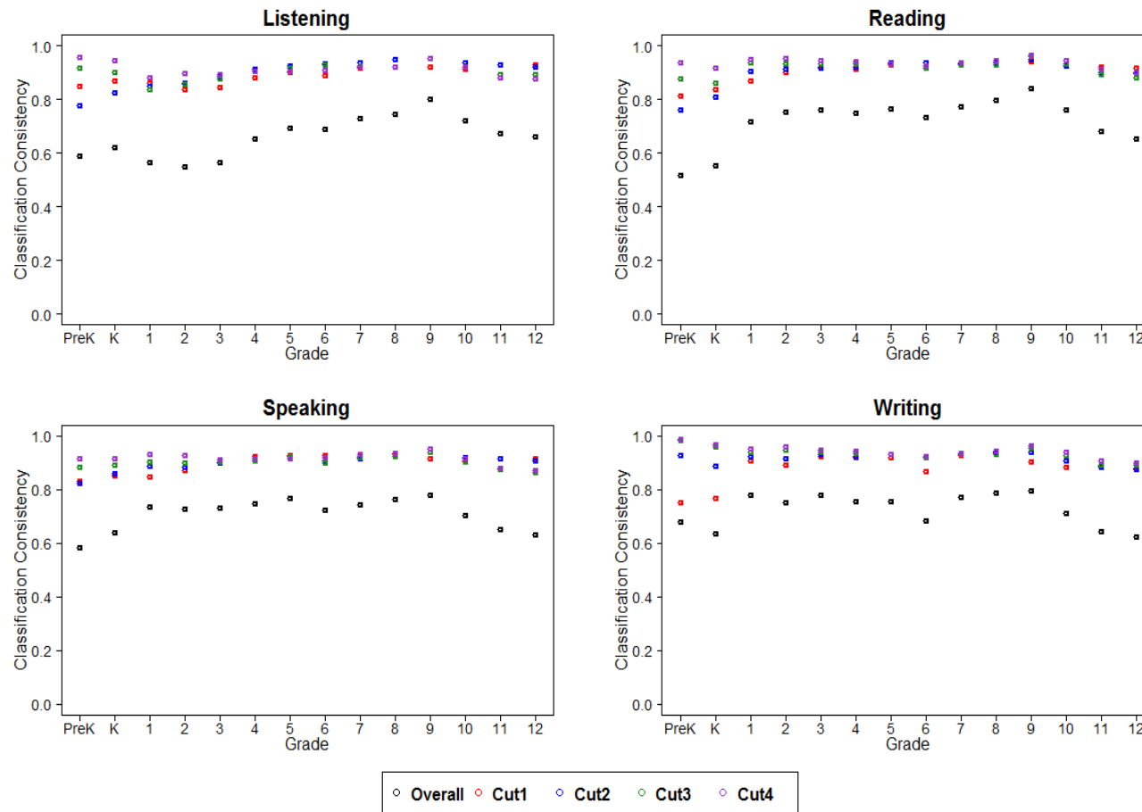
Figure S10.2: Screener Domain Level Classification Consistency
