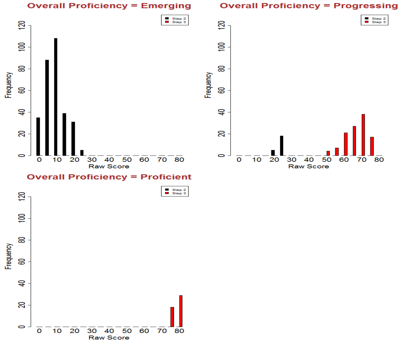
Figure S3.50: Screener Raw Score Distributions - Grade 8 Overall
