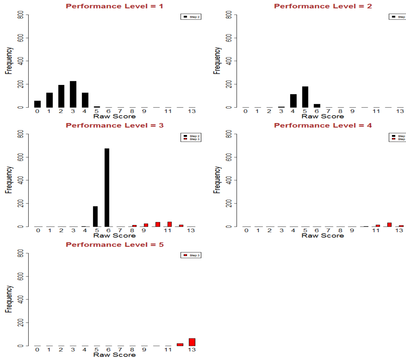
Figure S3.6: Screener Raw Score Distributions - Kindergarten Listening
