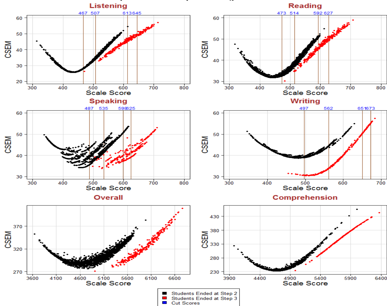
Figure S9.2: Screener Conditional Standard Error of Measurement for Kindergarten
