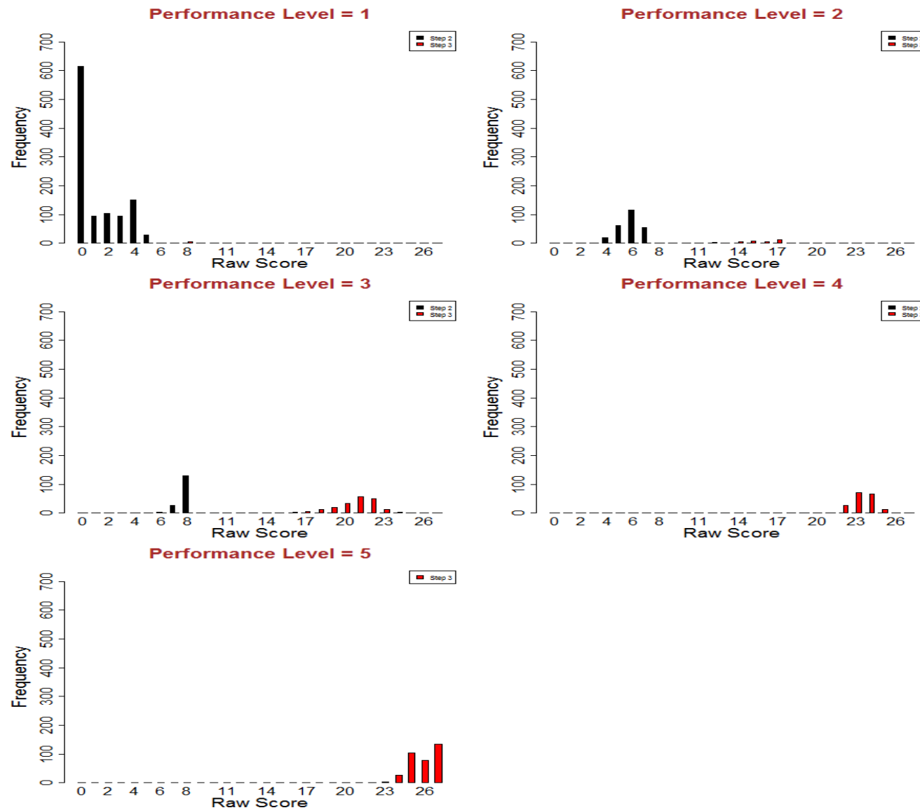
Figure S3.58: Screener Raw Score Distributions - Grade 10 Speaking
