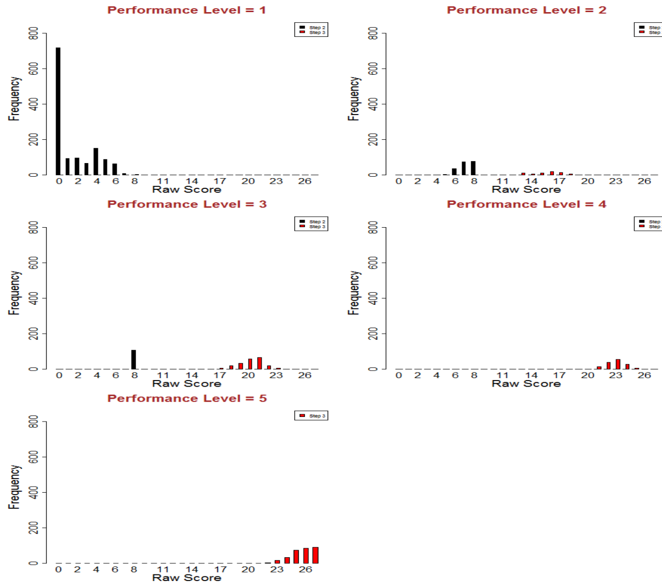
Figure S3.43: Screener Raw Score Distributions - Grade 7 Speaking
