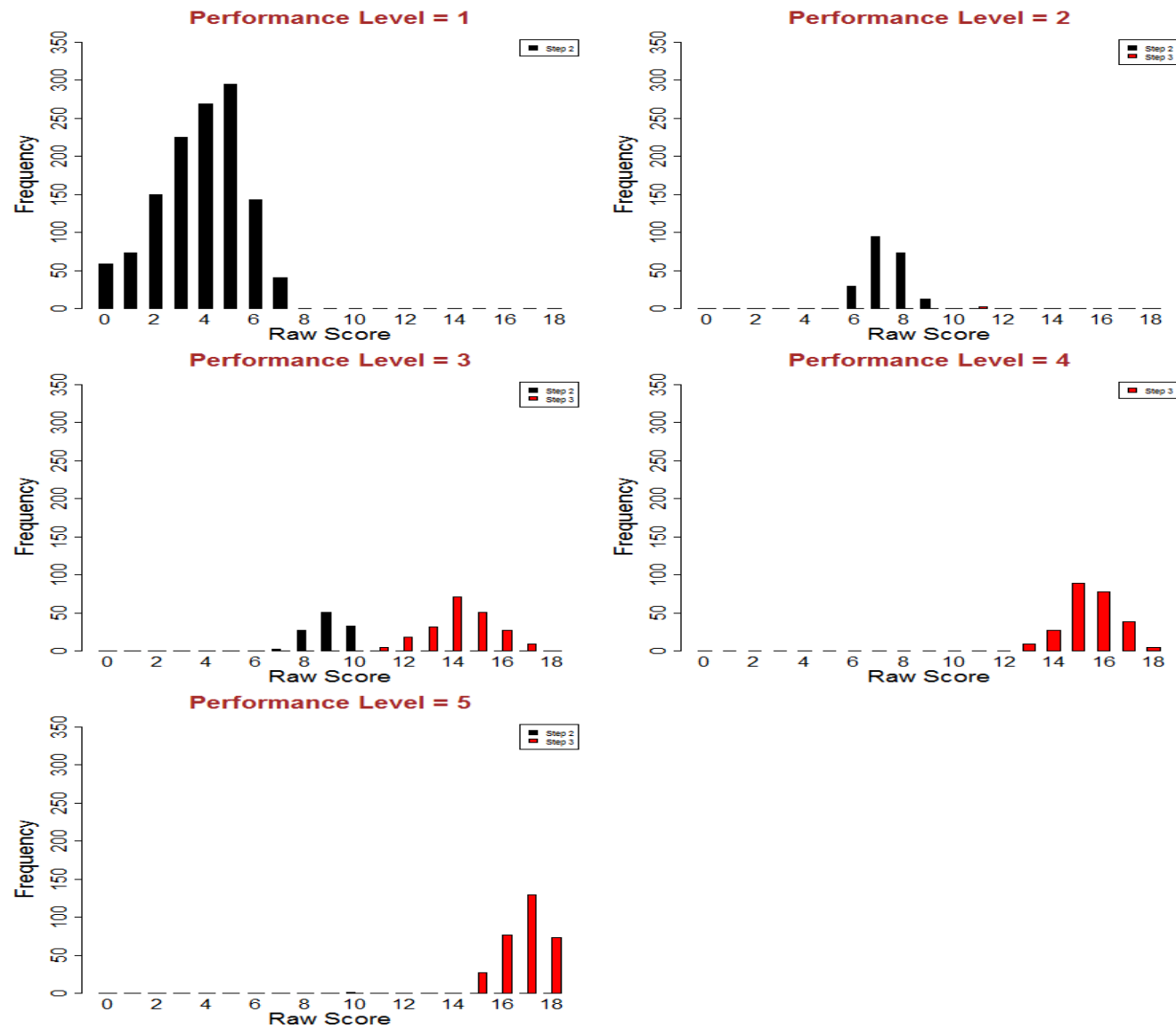
Figure S3.46: Screener Raw Score Distributions - Grade 8 Listening
