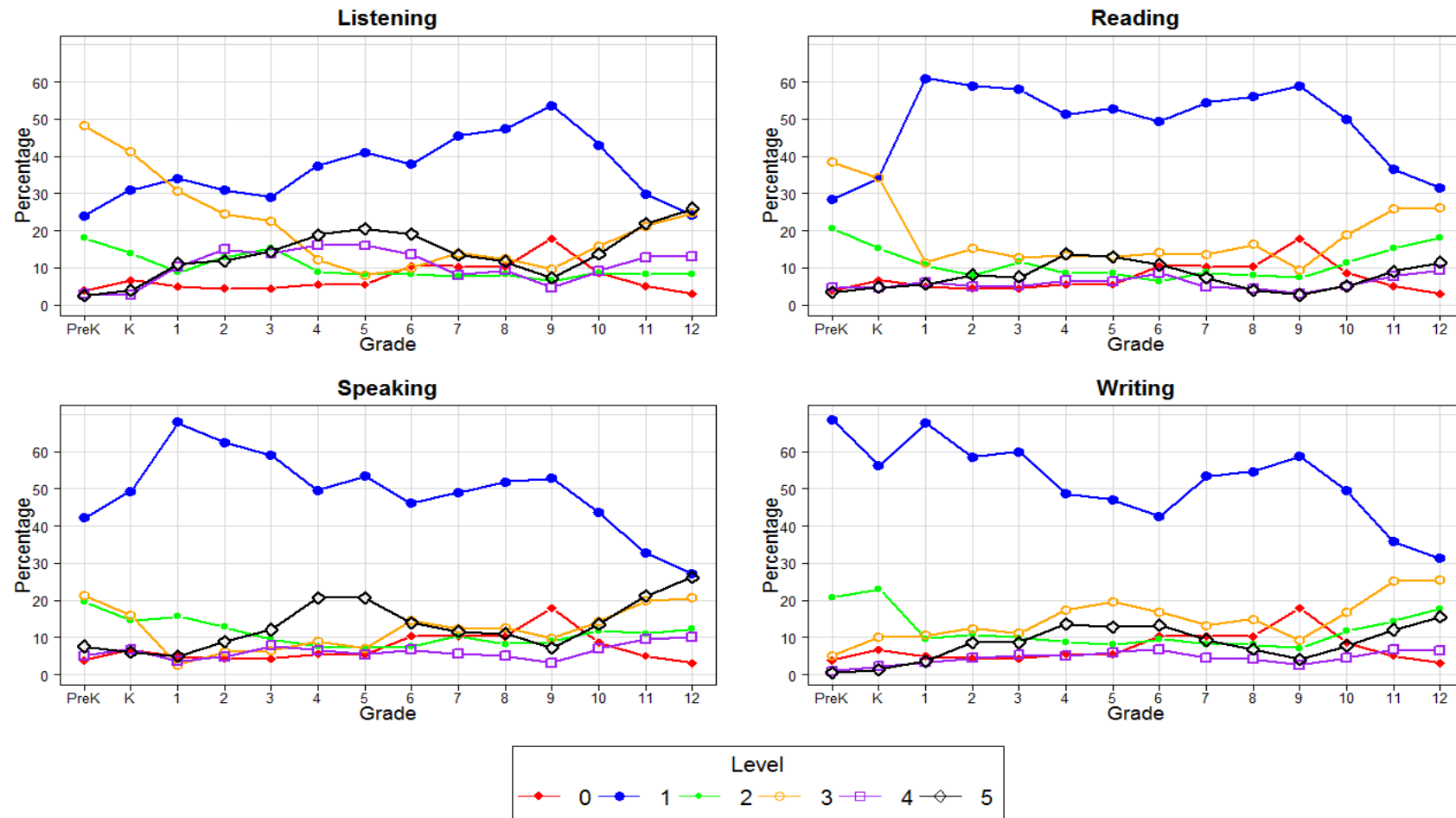
Figure S5.1: Screener Percentage of Students in Performance Levels
