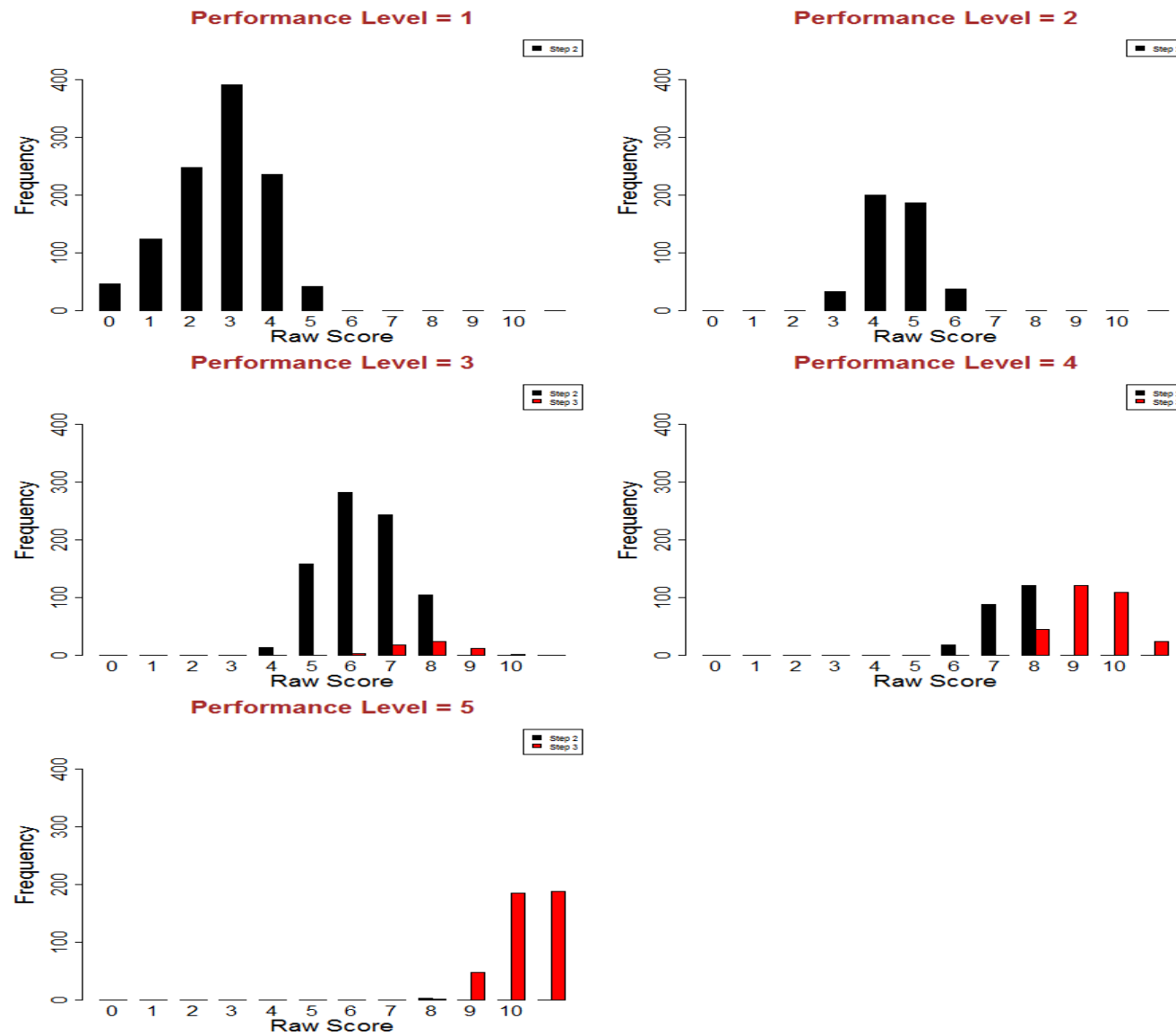
Figure S3.16: Screener Raw Score Distributions - Grade 2 Listening
