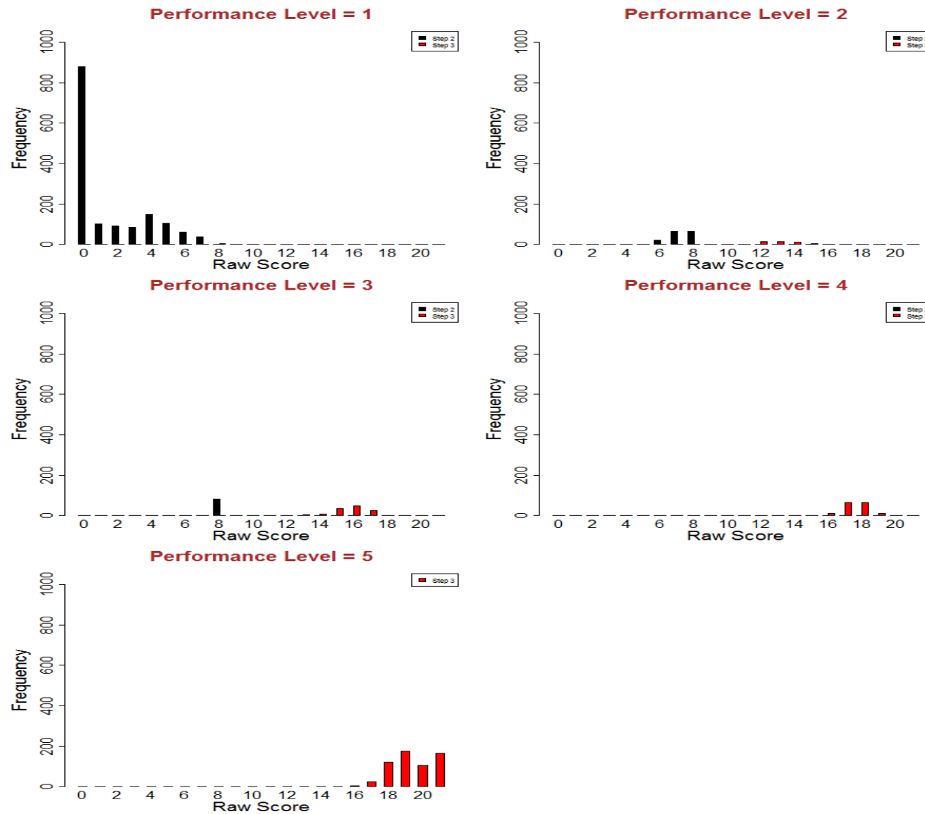
Figure S3.33: Screener Raw Score Distributions - Grade 5 Speaking
