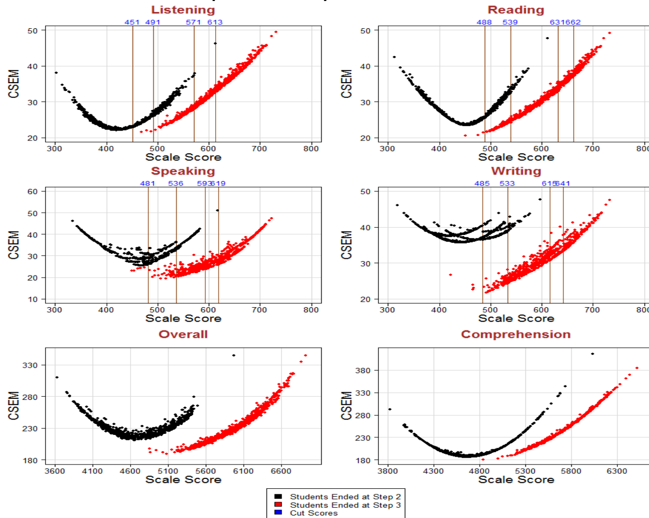
Figure S9.13: Screener Conditional Standard Error of Measurement for Grade 11
