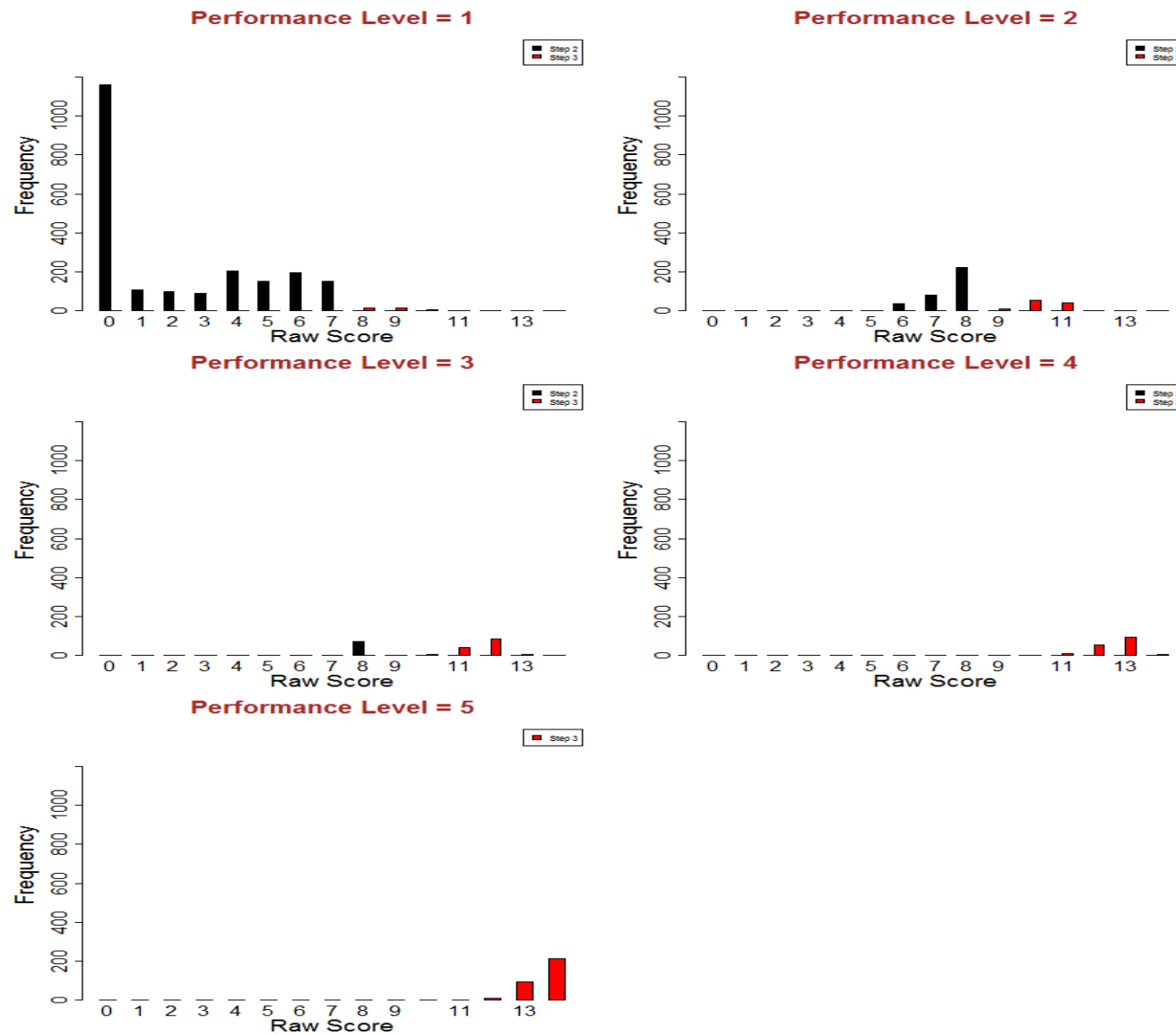
Figure S3.18: Screener Raw Score Distributions - Grade 2 Speaking
