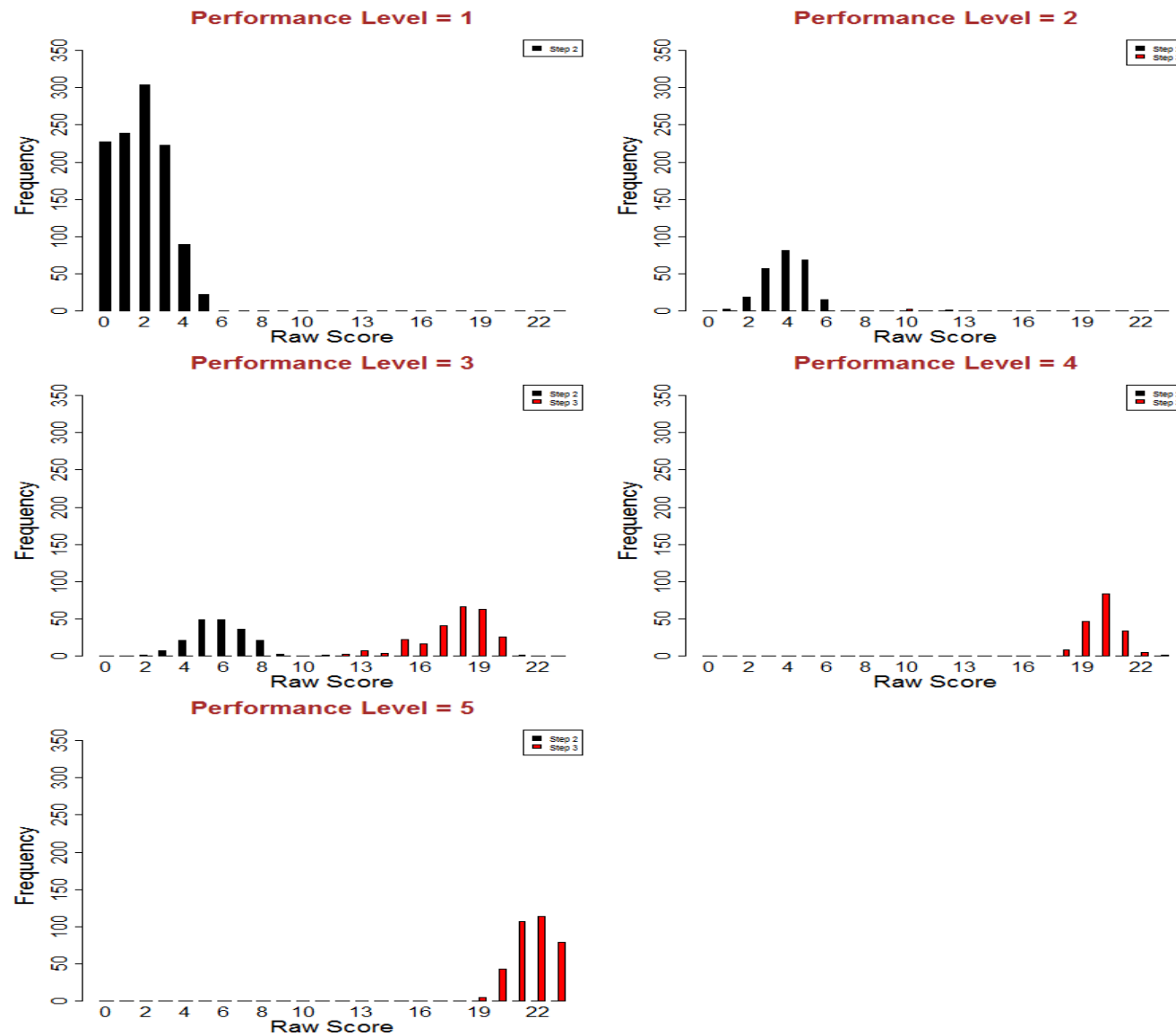
Figure S3.39: Screener Raw Score Distributions - Grade 6 Writing
