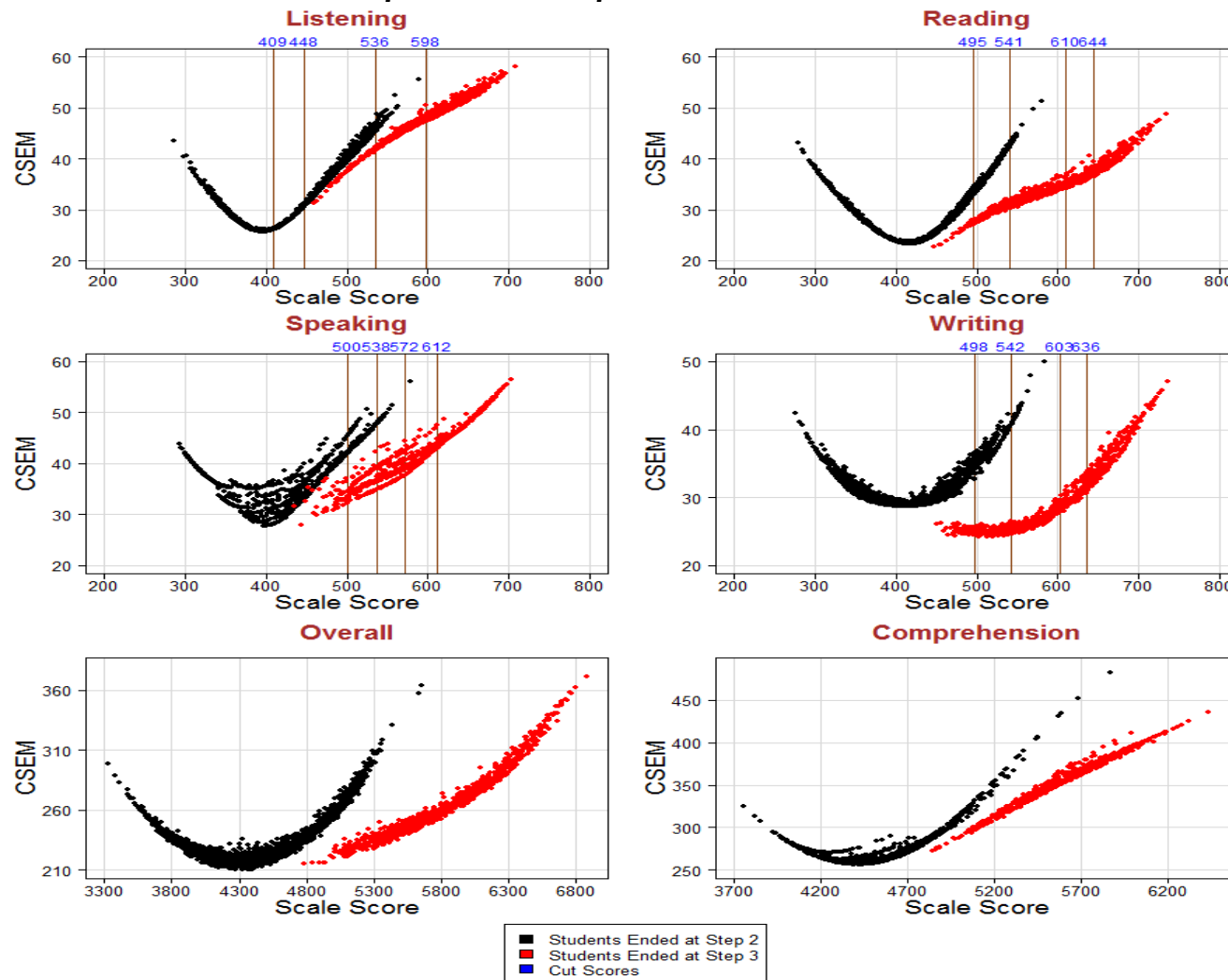
Figure S9.5: Screener Conditional Standard Error of Measurement for Grade 3
