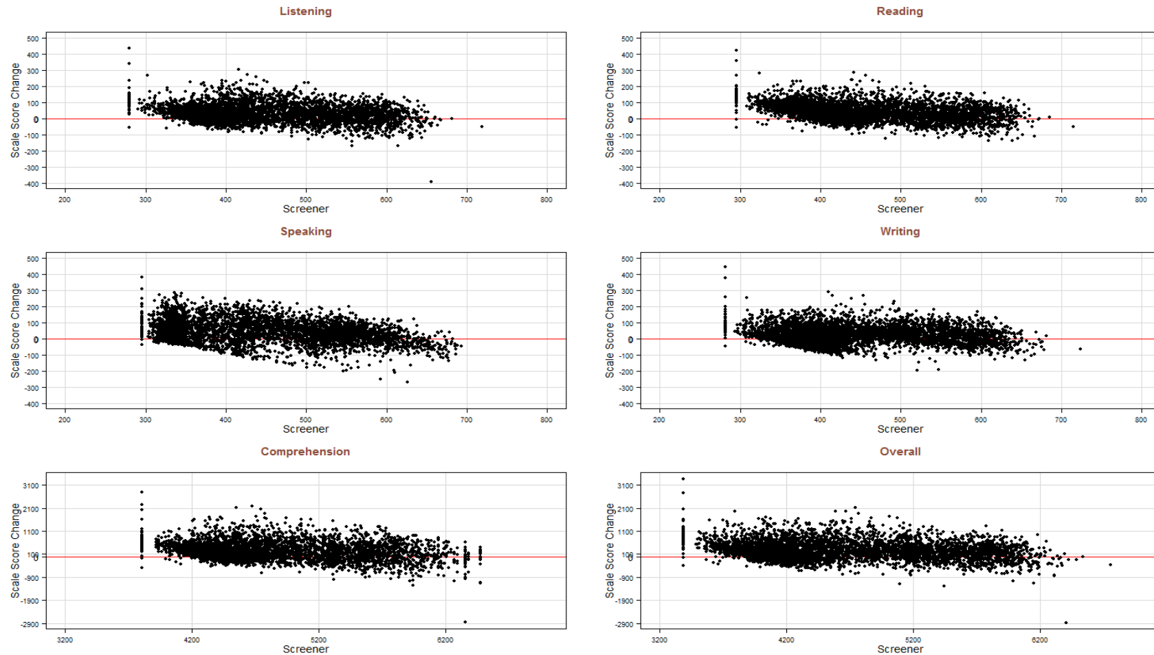
Figure S13.9: Scatter Plot of Scale Score Change from Screener to Summative for Grade Band 6-8
