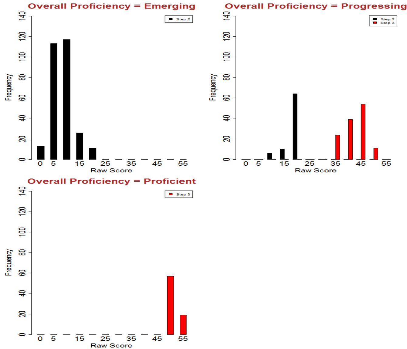
Figure S3.25: Screener Raw Score Distributions - Grade 3 Overall
