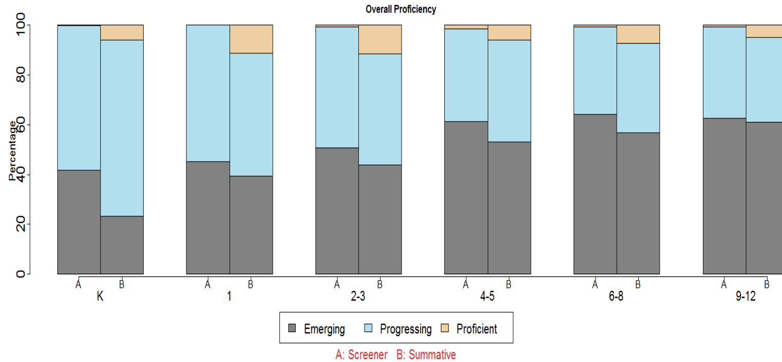
Figure S13.4: Percentages of Overall Proficiency Progress
