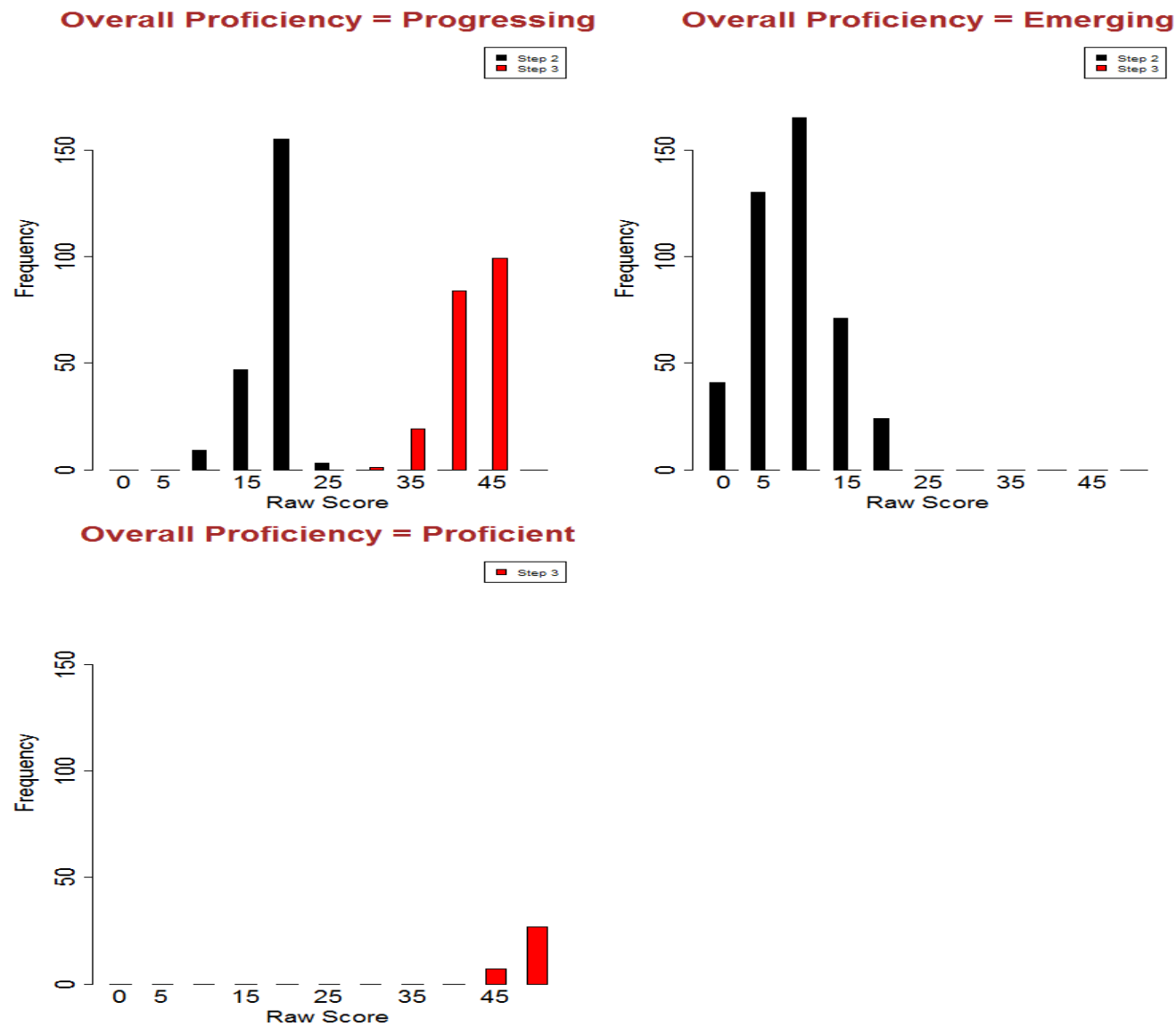
Figure S3.15: Screener Raw Score Distributions - Grade 1 Overall
