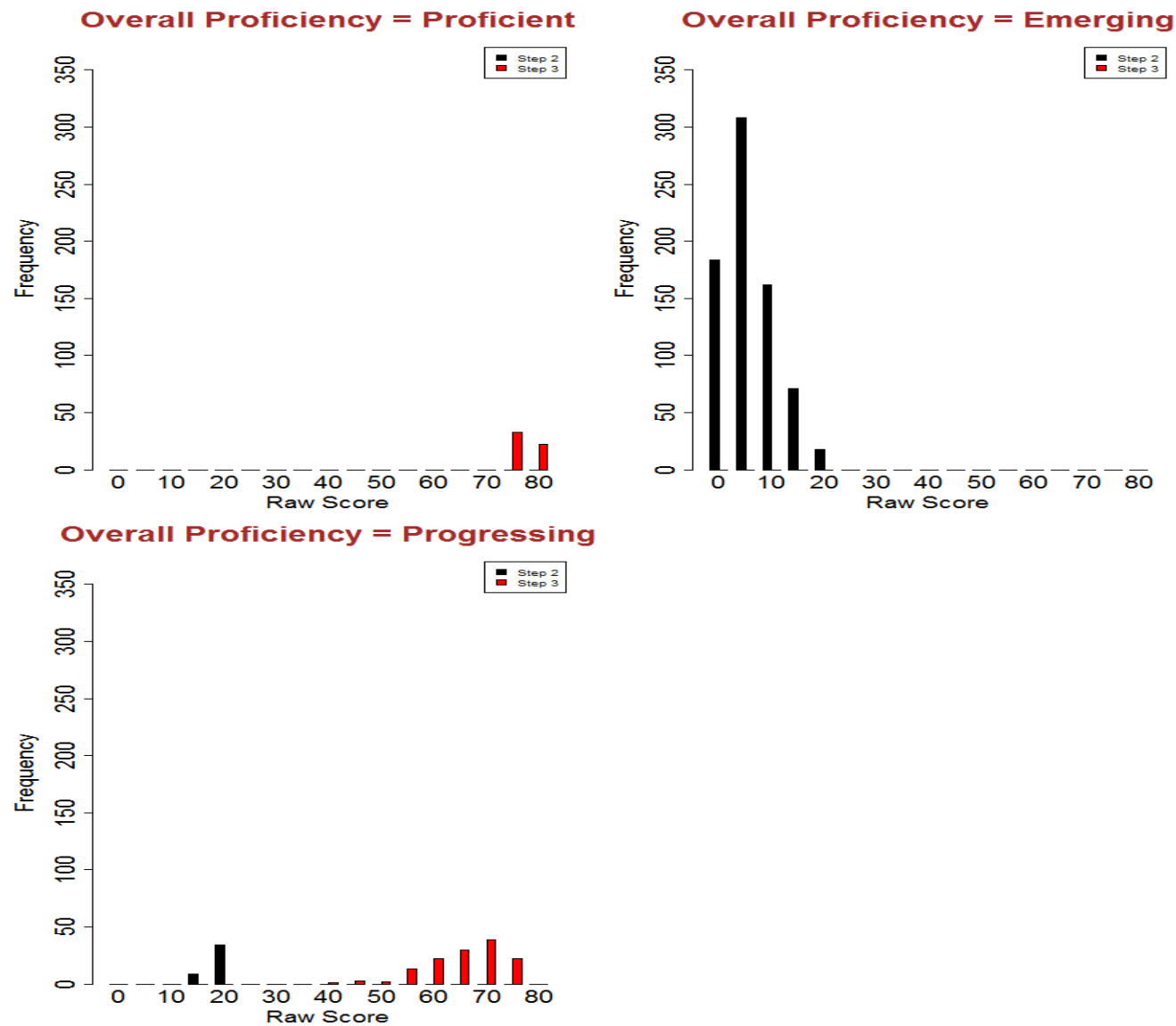
Figure S3.55: Screener Raw Score Distributions - Grade 9 Overall
