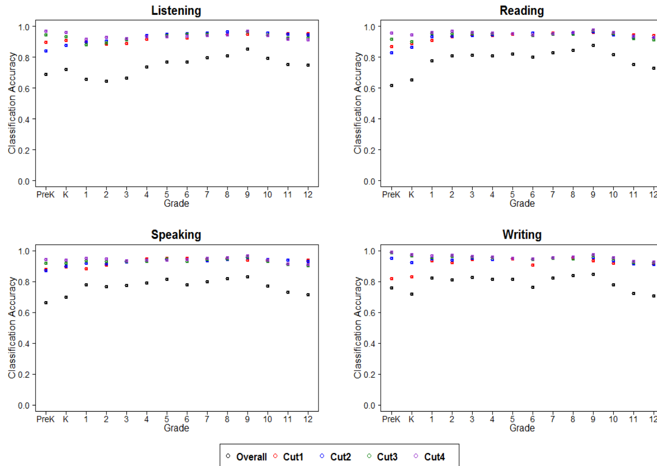
Figure S10.1: Screener Domain Level Classification Accuracy
