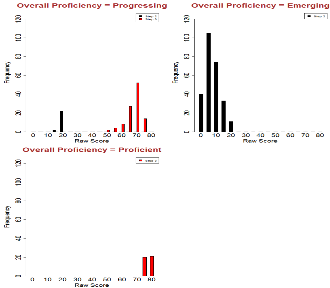
Figure S3.60: Screener Raw Score Distributions - Grade 10 Overall
