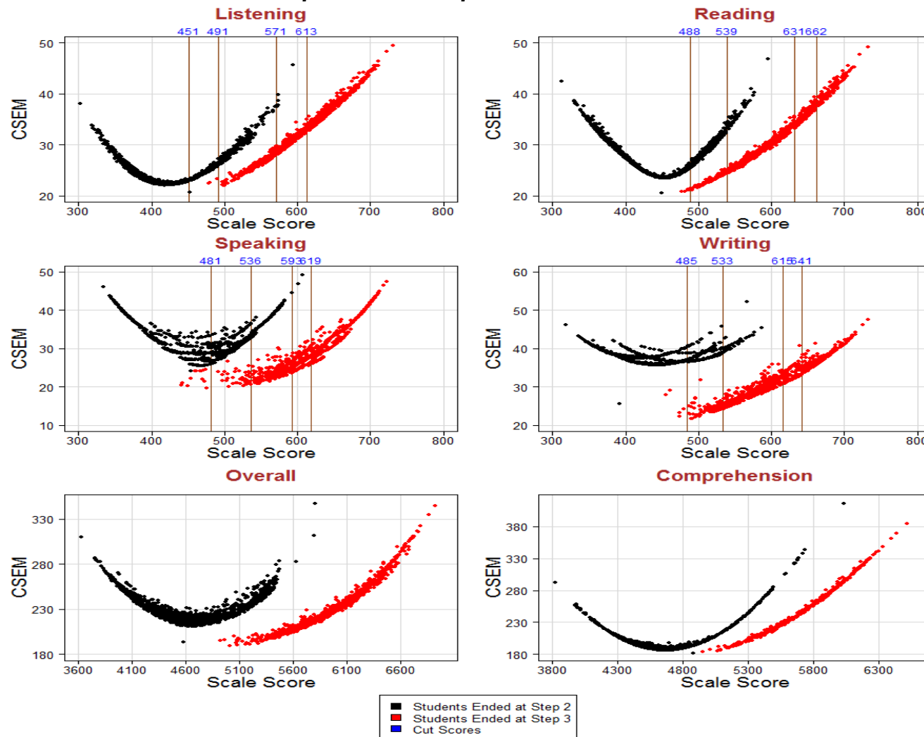
Figure S9.12: Screener Conditional Standard Error of Measurement for Grade 10
