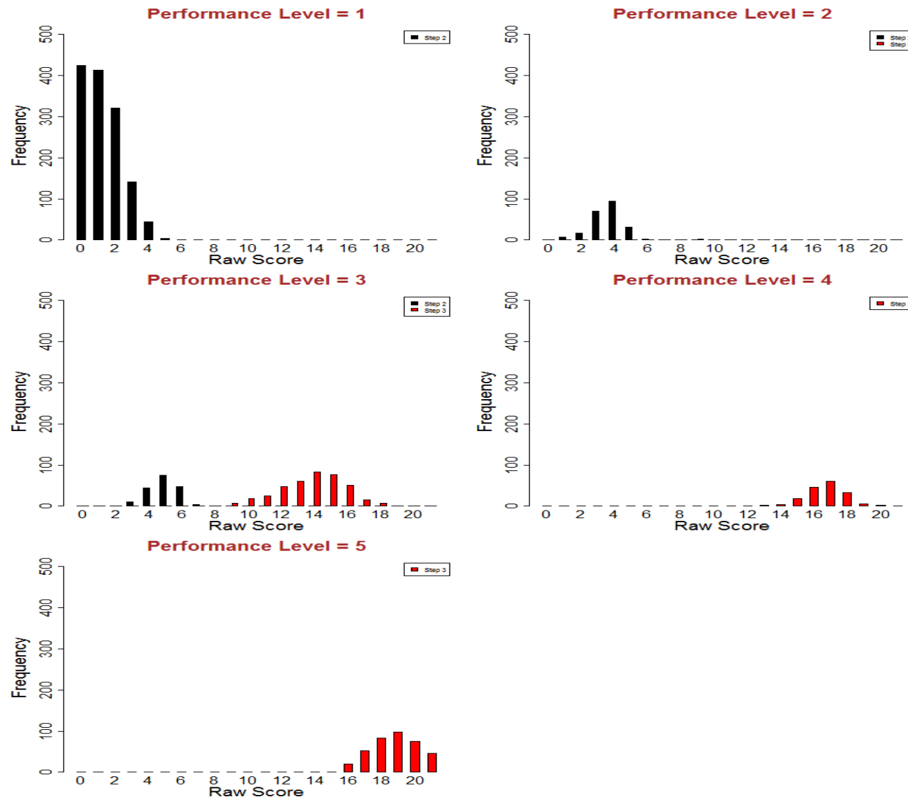
Figure S3.34: Screener Raw Score Distributions - Grade 5 Writing
