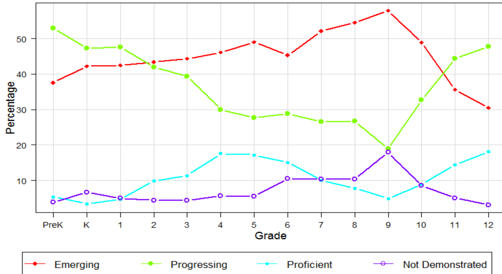
Figure S6.1: Screener Percentage of Students in Proficiency Categories
