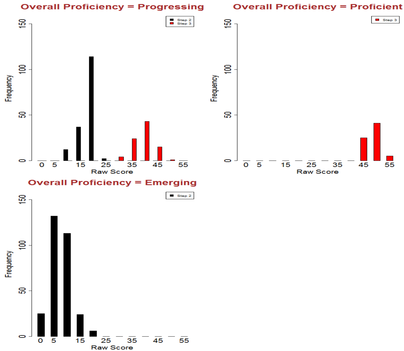
Figure S3.20: Screener Raw Score Distributions - Grade 2 Overall
