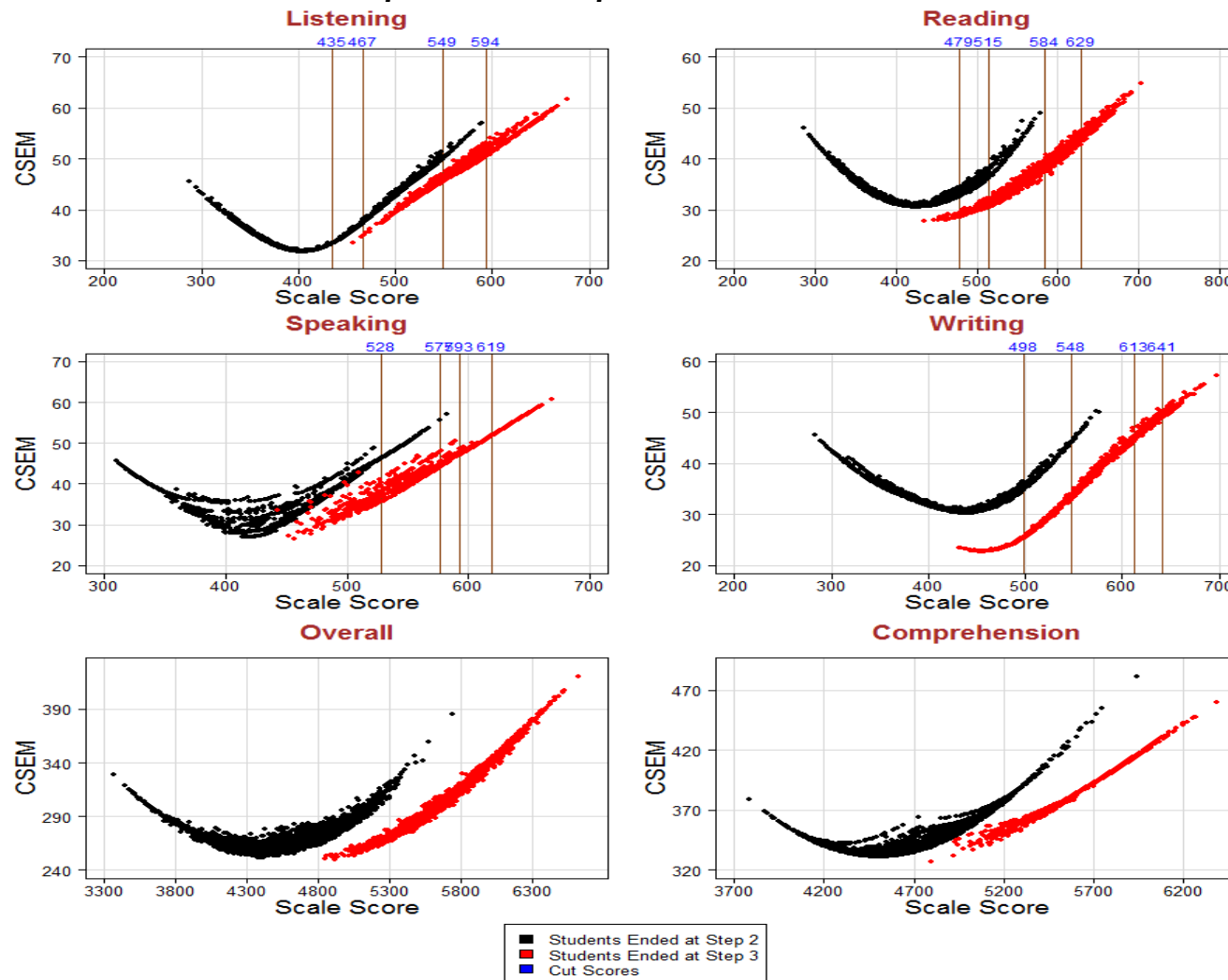
Figure S9.3: Screener Conditional Standard Error of Measurement for Grade 1
