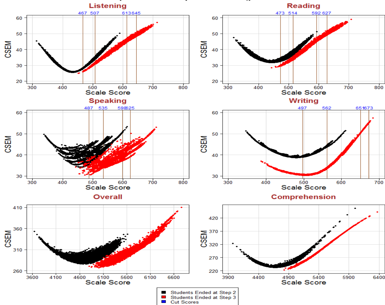
Figure S9.1: Screener Conditional Standard Error of Measurement for Pre-Kindergarten
