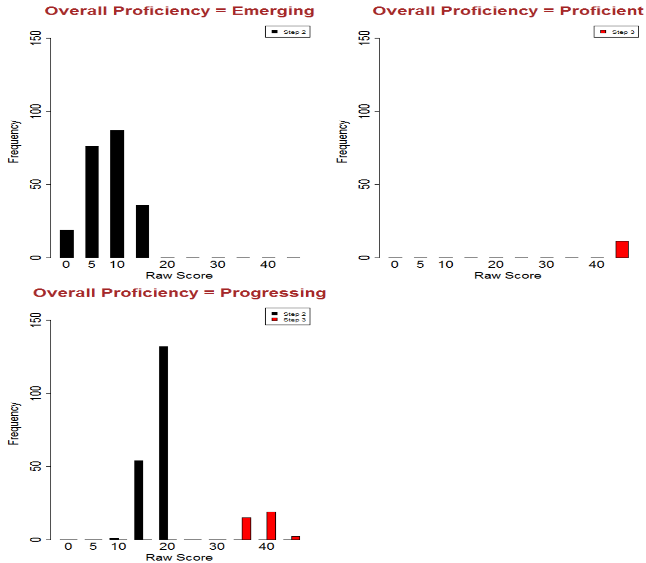
Figure S3.10: Screener Raw Score Distributions - Kindergarten Overall
