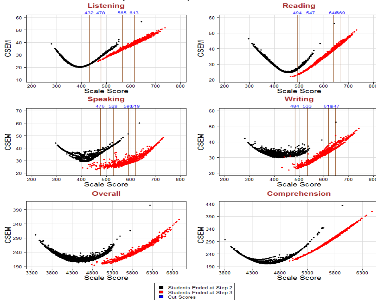
Figure S9.10: Screener Conditional Standard Error of Measurement for Grade 8
