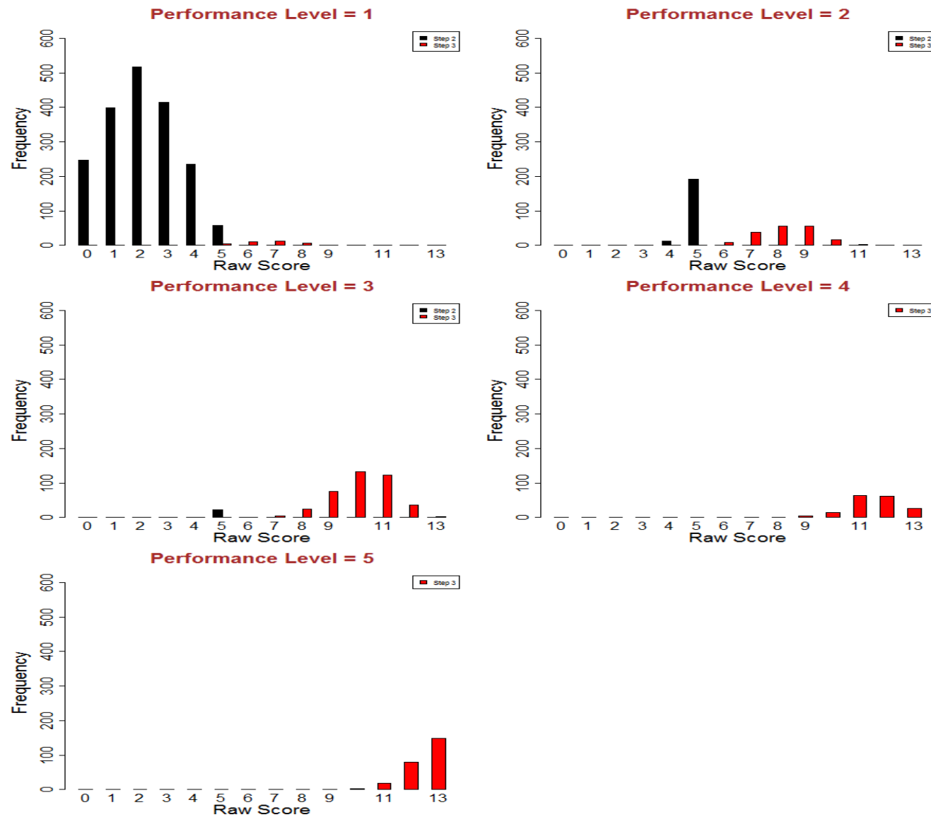
Figure S3.22: Screener Raw Score Distributions - Grade 3 Reading
